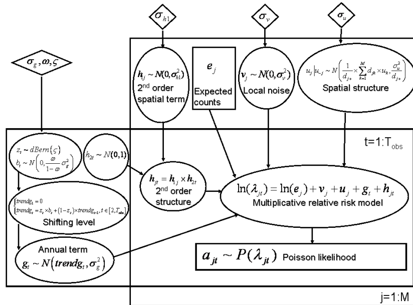
Figure 1. Model for avalanche occurrences. The circled nodes represent stochastic latent variables and the diamonds represent the overall parameters, while the rectangles indicate observed values.
