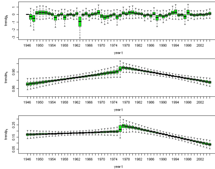
Figure 3. Box plots of the structured annual components separated from random noise in avalanche occurrences, mean runout altitude and probability of reaching the valley floor in France.
