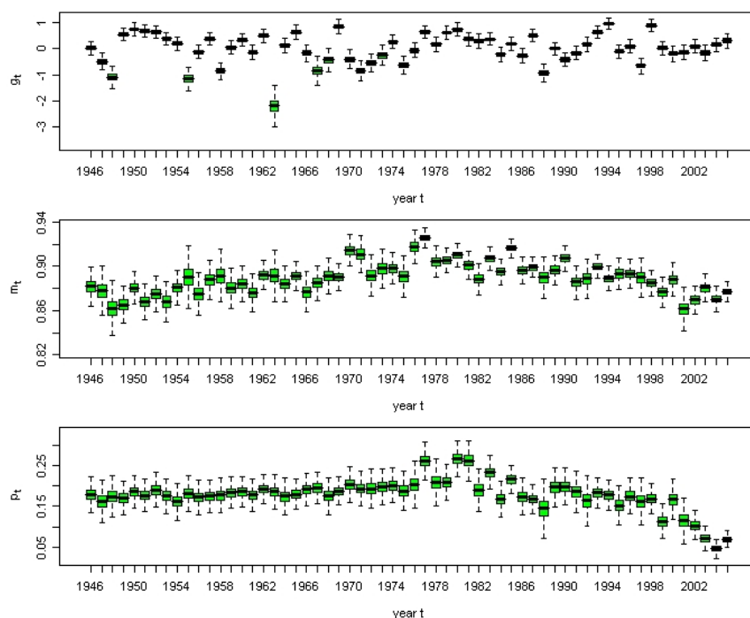
Figure 2. Box plots of the annual components in avalanche occurrences, mean runout altitude and probability of reaching the valley floor in France.
