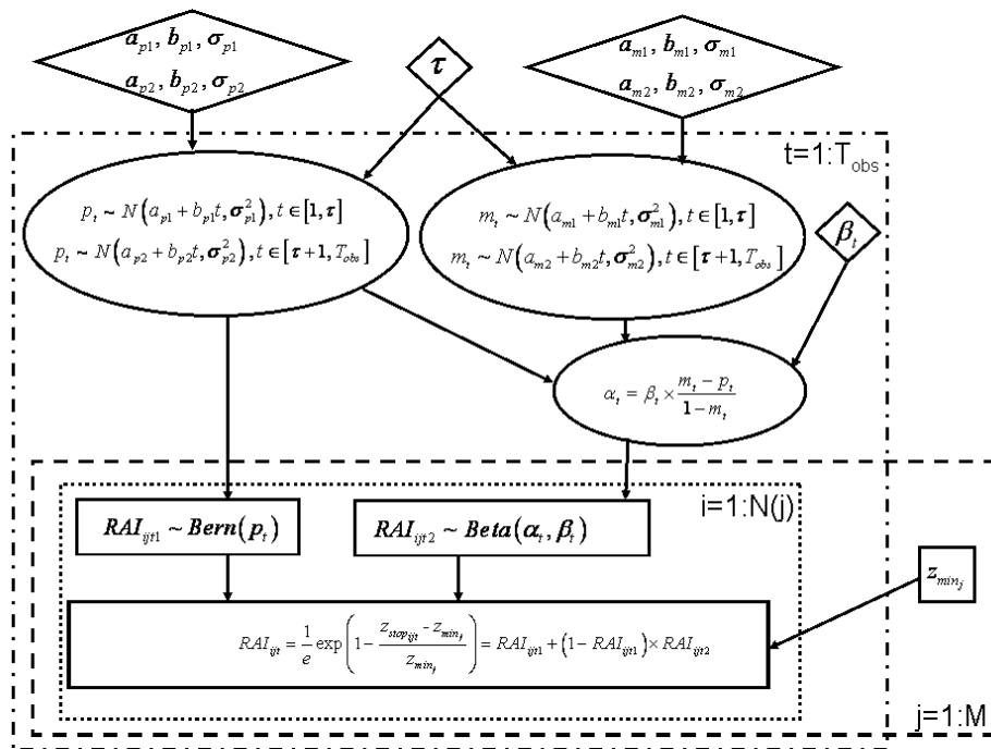
Figure 4. Change point model for mean and extreme snow avalanche runout altitudes
