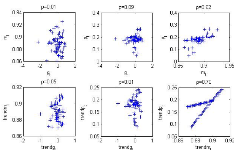
Figure 5. Scatter plots and empirical correlations between point estimates obtained with the two models
