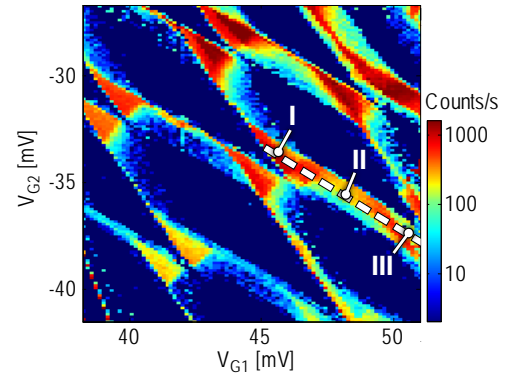
Figure 59: Charge stability diagram of the double quantum dot, recorded by counting electrons entering and leaving the structure. The data was taken at DQD bias voltage V_{DQD-SD} = 600 \mu\text{V} and B = 0 \text{ T} . The dashed line marks the region of cotunneling used for measuring single-electron Aharonov-Bohm interference.
