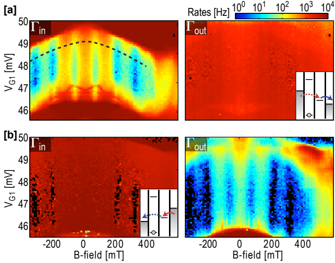
Figure 61: (a) Tunneling rates for electrons entering ( \Gamma_{\text{in}} ) and leaving ( \Gamma_{\text{out}} ) the DQD, measured versus electrochemical potential of QD1 and magnetic field. The y-axis corresponds to sweeps along the dashed line in Fig. 59. Within the cotunneling region, \Gamma_{\text{in}} shows clear B-field periodicity, while \Gamma_{\text{out}} remains constant. This is in agreement with the picture where only the electrons tunneling from source to QD2 encircle the Aharonov-Bohm ring, while electrons leaving to drain remain unaffected by the applied B-field. (b) Same as (a), but with reverse bias over the DQD. Here, the roles of \Gamma_{\text{in}} and \Gamma_{\text{out}} are inverted. Adapted from Ref. [69].
