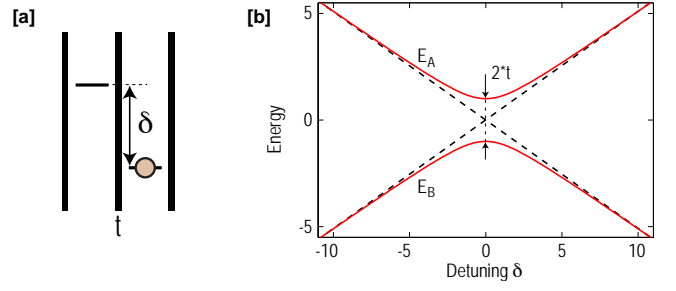
Figure 37: (a) Schematics of a tunnel coupled two-level system. (b) The energy levels of the two-level system, calculated from Eq. (71) with t = 1 . The dashed lines show the energy levels for isolated QDs ( t = 0 ).
