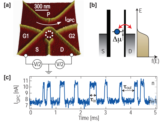
Figure 9: (a) Quantum dot with integrated charge read-out investigated in this section. (b) Schematic drawing depicting the electrochemical potentials of the system. By making the barrier between source and the QD very opaque, electron tunneling is only possible between the QD and the drain lead. (c) Current through the QPC as a function of time, showing a few electrons tunneling into and out of the QD. The lower current level corresponds to a situation where the QD holds one excess electron. Transitions between the two levels occur whenever an electron enters or leaves the QD. The quantities \tau_{\text{in}} and \tau_{\text{out}} specify the time it takes for an electron to tunnel into and out of the dot, respectively.
