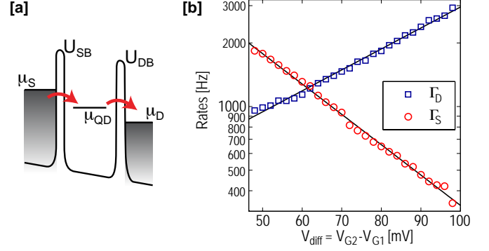
Figure 14: (a) Potential landscape of the QD when a fixed bias voltage is applied between the source and drain contacts. (b) Tunneling rates \Gamma_{\text{S}}/\Gamma_{\text{D}} measured versus V_{\text{diff}} = V_{\text{G2}} - V_{\text{G1}} . The solid lines are fits to Eq. (24) in the text. The measurements were performed by sweeping both gate voltages V_{\text{G1}} , V_{\text{G2}} , with V_{\text{G1}} = -0.142 - V_{\text{G2}} .
