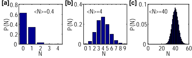
Figure 29: Current distribution functions, extracted for different values of t_0 . The underlying data is the same in all three figures. For very short t_0 [case (a)], the distribution clearly has different properties compared to case (c).
