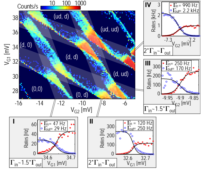
Figure 46: Charge stability diagram of the DQD, together with a possible spin configuration extracted from analyzing rates for electrons tunneling into and out of the QDs. The numbers do not refer to the absolute DQD electron population but to the excess electron population relative to the configuration marked by (0,0). Cases I-II shows degeneracies measured when filling QD2, cases III-IV refer to filling of QD1. The measurements shown in cases I-IV were taken with zero bias over the DQD in order to minimize the influence of cotunneling.
