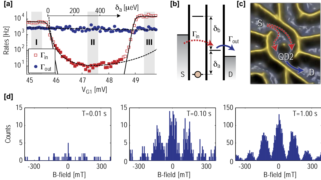
Figure 60: (a) Tunneling rates for electrons entering (red) and leaving (blue) the DQD, measured along the dashed white line of cotunneling in Fig. 59(a). The upper x-axis shows \delta , the potential difference between the state in QD2 and the occupied state of QD1. The solid lines are tunneling rates expected from sequential tunneling, while the dashed line is a fit to the cotunneling model of Eq. (74) with parameters \Gamma_{S_a} = 6.4 kHz, \Gamma_{S_b} = 14 kHz, t_a = 8.3 \mu\text{eV} and t_b = 13 \mu\text{eV} . The data was taken with B = 340 mT. (b) Schematic drawings of the energy levels of the DQD at position II in (a). The energy levels of QD1 are shifted so that the electron in QD1 is trapped due to Coulomb blockade. Electron transport from source to QD2 is still possible through virtual processes. (c) The tunneling processes depicted in the double quantum dot structure. When both barriers between the QDs are kept open, the cotunneling electron may take any arm when going from source to QD2. (d) Number of electrons arriving at QD2 within the fixed period of time indicated in the upper-right corner, measured as a function of magnetic field. The data was taken at point II in (a). The count rate shows an oscillatory pattern with a visibility higher than 90%. Adapted from Ref. [69].
