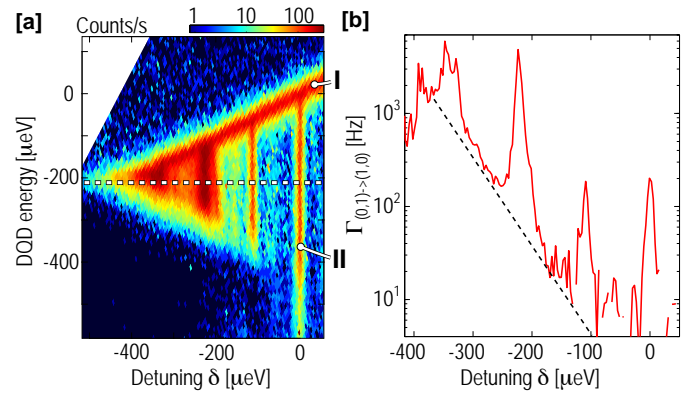
Figure 50: (a) Same as Fig. 49(a), but with the gate voltages converted to average energy and detuning of the double quantum dot. The line coming from tunneling between QD1 and the lead (case I) is considerably broader than the lines due to interdot transitions (case II). (b) Rate for the interdot transition (0,1) \rightarrow (1,0) , measured along the dashed line in (a). The peaks come from resonant tunneling through excited states in either QD. The inelastic tunneling between resonant peaks increases strongly with increased detuning. The dashed line is a guide to the eye depicting exponential increase.
