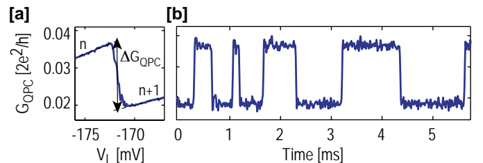
Figure 3: (a) QPC conductance measured versus voltage on gate L. At V_L = -172 \text{ mV} an electron is added to the QD, leading to a decrease of G_{\text{QPC}} . (b) Time trace of the QPC conductance measured at V_L = -172 \text{ mV} , showing a few electrons tunneling into and out of the QD. The upper level corresponds to a situation with n electrons on the QD. Adapted from Ref. [5].
