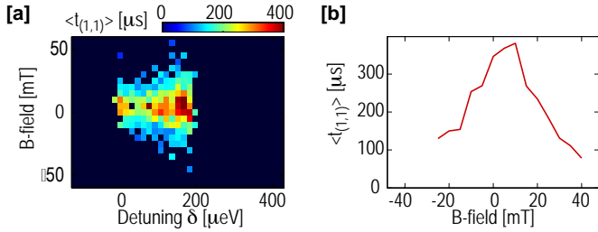
Figure 48: (a) Average time spent in the (1,1) state, measured vs DQD detuning and magnetic field. The third level in the QPC conductance traces corresponding to the (1,1) state is only visible in the region 0 < \delta < E_{ST} \sim 200 \mu\text{eV} . The data was taken along the dashed line in Fig. 47(d). (b) Cross-section of the graph in (a), taken at \delta = 170 \mu\text{eV} . The time t_{(1,1)} falls off quickly with increased B-field and drops below the time resolution of the detector as |B| > 30 mT.
