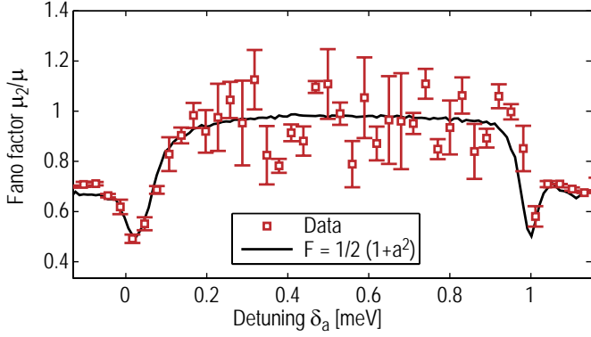
Figure 45: Fano factor for electron transport in the cotunneling regime of Fig. 39. The data was extracted from traces of length T = 30 s. The solid line is the result of Eq. (78), which assumes independent tunneling events. The minima in Fano factor occur at positions where the tunneling rates \Gamma_{\text{in}} and \Gamma_{\text{out}} are equal (see Fig. 39). The error bars show standard error, extracted by splitting the data into six subsets of length T = 5 s and evaluating the noise for each subset. Adapted from Ref. [66].
