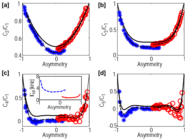
Figure 26: (a-d) Normalized cumulants C_n/C_1 versus dot asymmetry, a = (\Gamma_{\text{in}} - \Gamma_{\text{out}})/(\Gamma_{\text{in}} + \Gamma_{\text{out}}) . The solid lines are theoretical predictions assuming a perfect detector, C_2/C_1 = (1 + a^2)/2 , C_3/C_1 = (1 + 3a^4)/4 , C_4/C_1 = (1 + a^2 - 9a^4 + 15a^6)/8 and C_5/C_1 = (1 + 30a^4 - 120a^6 + 105a^8)/16 . The dashed lines show the cumulants calculated from the model defined by Eq. (50) in the text. The inset in (c) shows the variation of the total tunneling rate \Gamma_{\text{tot}} = \Gamma_{\text{in}} + \Gamma_{\text{out}} for the different measurement points. Adapted from Ref. [60].
