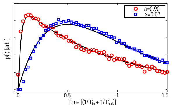
Figure 23: Distribution of times needed for one electron to pass through the QD, measured with both symmetric and asymmetric tunnel couplings. To make qualitative comparisons of the two distributions easier, the two curves are plotted with different vertical scaling. The time scale is normalized to the average time needed for one electron to pass the dot.
