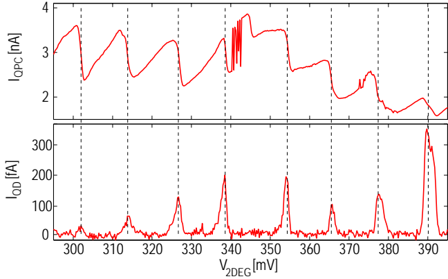
Figure 2: Current in the QPC and the QD for the structure shown in Fig. 1(a), measured vs voltage on the 2DEG. A second gate is tuned simultaneously to keep the potential of the QPC roughly constant during the sweep. As the voltage of the 2DEG is lowered, electrons are unloaded from the QD. At each transition there is a corresponding increase in the QPC conductance. At the same gate voltages, sequential tunneling gives rise to peaks in the QD current.
