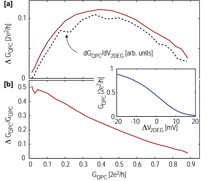
Figure 6: (a) Change of QPC conductance as one electron enters the QD, measured for different values of average QPC conductance. The dashed line is the numerical derivative of the QPC conductance with respect to gate voltage. The change is maximal at G_{\text{QPC}} = 0.4 \times 2e^2/h , which coincides with the steepest part of the QPC conductance curve [see inset in (b)]. (b) Relative change of QPC conductance for one electron entering the QD, defined as (G_{\text{high}} - G_{\text{low}})/G_{\text{high}} . The relative change increases with decreased G_{\text{QPC}} , reaching above 50% at G_{\text{QPC}} = 0.02 \times 2e^2/h . The inset shows the variation of G_{\text{QPC}} as a function of gate voltage. Adapted from Ref. [5].
