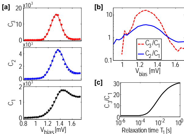
Figure 25: (a) First, second and third cumulants of the distribution of charge fluctuations. The symbols show values extracted from the experimental data, while the solid lines are calculated from the model given in the text. Fitting parameters are: \Gamma_A = 1.6 kHz, \Gamma_B = 20.5 kHz, \Gamma_{\text{right}}^A = 4.6 kHz, \Gamma_{\text{right}}^B = 310 Hz, T_1 = 8 ms and \mu_A - \mu_B = 13 \mu\text{eV} . The electronic temperature was 400 mK. (b) Normalized cumulants C_3/C_1 and C_2/C_1 versus bias voltage. The noise is clearly super-Poissonian in the central region of the graph. (c) Calculated maximal value of C_3/C_1 as a function of the relaxation time between the two states. The values are calculated by varying the relaxation time while keeping the other parameters to the values given by the fit shown in (a). The maximum value C_3/C_1 extracted from the experimental data is 15.9. Adapted from Ref. [20].
