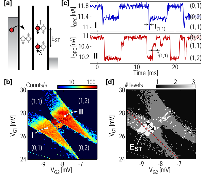
Figure 47: (a) Sketch of a DQD in the regime of Pauli spin blockade. If the electron entering QD1 has the same spin orientation as the electron sitting in QD2, transport is blocked until either electron flips its spin to allow a singlet state to form in QD2. (b) Charge stability diagram measured by counting electrons entering the DQD. The numbers refer to the assumed excess charge population relative to a state where both QDs have zero spin. The data was extracted from QPC conductance traces of length T = 0.5 s, taken with V_{\text{DQD-SD}} = 600 \mu\text{V} and V_{\text{QPC-SD}} = 400 \mu\text{V} . (c) QPC conductance traces, taken at the points marked in (b). For both positions, a third level appears which we attribute to the transition (1,1) \rightarrow (0,2). (d) Regions of the charge stability diagram of (b) where the charge detector finds more than two levels in the QPC conductance traces. In the spin blockade model of (a), the width of regions with three levels corresponds to the singlet-triplet spacing in QD2.
