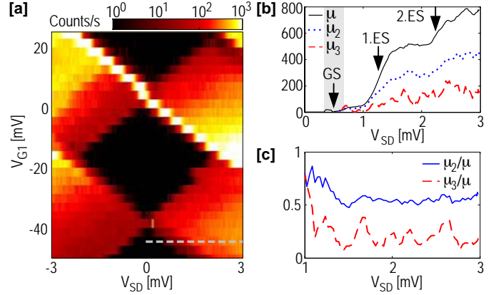
Figure 21: (a) Average number \mu of electrons entering the QD, measured as a function of the gate voltage V_{G1} and the bias voltage V_{SD} . Far from the edges of the Coulomb blockade region, i.e. for |\pm eV_{SD}/2 - E_d| \gg k_B T , the fluctuations of n are directly related to current fluctuations. The dashed line correspond to the cross-section shown in panel (b). (b) Three first moments of the fluctuations of n as a function of the bias voltage V_{SD} and at a given gate voltage V_{G1} = -44 mV. The ground state (GS) as well as two excited states (ES) are clearly visible. The moments are scaled so that \mu corresponds to the number of electrons entering the QD per second. In the gray region, the condition |\pm eV_{SD}/2 - \mu_n| \gg k_B T is not valid, and the number of electrons entering the QD cannot be taken as the current flowing through the QD. The width of this region is 9 \times k_B T/e \approx 300 \mu\text{V} , determined from the width for which the Fermi distribution is between 0.01 and 0.99. (c) Normalized second and third moments as a function of the bias voltage V_{SD} and at a given gate voltage V_{G1} = -44 mV. Adapted from Ref. [40].
