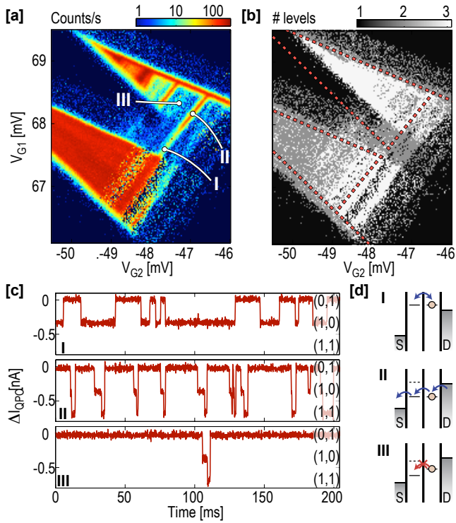
Figure 49: (a) Charge stability diagram of the DQD measured by counting electrons entering the DQD. The data was taken with V_{DQD-SD} = -700 \mu V and V_{QPC-SD} = 300 \mu V . (b) Number of levels in the QPC conductance traces, extracted from the same data as in (a). The dashed lines show the extension of the triangle expected from the applied bias and the capacitive lever arms of the gates. (c) QPC conductance traces, taken at three positions marked in (a). In case I, the tunneling is due to equilibrium fluctuations between QD1 and QD2. In cases II-III, a current flows through the DQD. (d) Energy level diagrams depicting the DQD configuration for the three position in (a,c).
