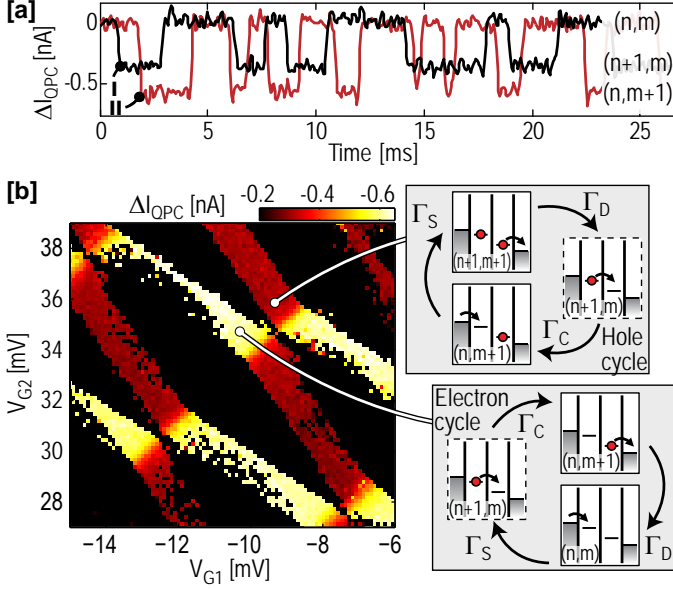
Figure 36: (a) Typical time traces of the QPC current from configurations I and II in Fig. 35. (b) Change of QPC current \Delta I_{\text{QPC}} as one electron enters the DQD, extracted from the same set of data as shown in Fig. 35. The two levels correspond to the QPC detector registering electron tunneling in QD1 and QD2, respectively. The energy level diagrams describe the hole and the electron cycle of sequential transport within the finite bias triangles. Adapted from Ref. [66].
