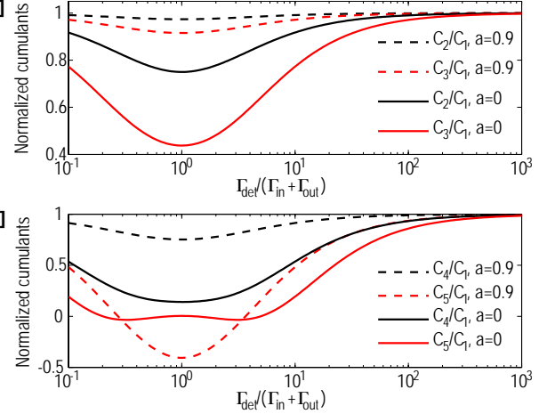
Figure 28: Higher cumulants versus relative detection bandwidth \Gamma_{\text{det}}/(\Gamma_{\text{in}} + \Gamma_{\text{out}}) , calculated from the model in Fig. 27(b). The cumulants are normalized with respect to the results for the infinite-bandwidth case. The influence of the finite bandwidth is maximal when the asymmetry a = (\Gamma_{\text{in}} - \Gamma_{\text{out}})/(\Gamma_{\text{in}} + \Gamma_{\text{out}}) is zero. Adapted from Ref. [60].
