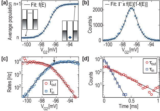
Figure 10: (a) Average dot population versus voltage on gate G2 . The fit shows the Fermi distribution function with T = 230 mK. (b) Counts per second for the same data as in (a). The data was fit to Eq. (14), giving \Gamma = 9.2 kHz and T = 230 mK. (c) Tunneling rates for electrons entering (squares) and leaving (circles) the QD, extracted from the same set of data as in (a, b). The solid lines are the results of Eqs. (10-11) in the text, with \Gamma = 9.2 kHz and T = 230 mK. (d) Distribution of tunneling times for electrons entering (squares) and leaving (circles) the QD, extracted at V_{G2} = -96.3 mV [marked by arrow in (c)]. The solid lines show the exponential behavior given by Eq. (9) in the text, with \Gamma_{in} = 1/\langle\tau_{in}\rangle = 7.2 kHz, \Gamma_{out} = 1/\langle\tau_{out}\rangle = 2.0 kHz. The length of the time trace for the data shown in the figure is 0.5 s.
