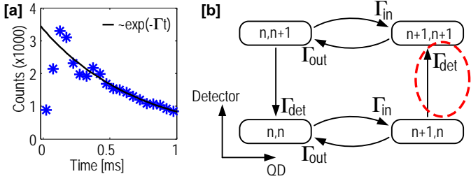
Figure 27: (a) Probability density of time needed for an electron to tunnel into the dot. Note the sharp decrease in counts for t < 100 \mu\text{s} due to the finite bandwidth of the detector. The black curve is a long-time exponential fit with \Gamma = 1.39 \text{ kHz} . (b) Model for the dot-detector system. A state (n, m) corresponds to n electrons on the dot while the detector at the same time is measuring m electrons. Adapted from Ref. [60].
