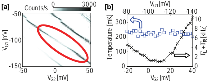
Figure 11: (a) Counts per second versus V_{G1} and V_{G2} . For low values of V_{G1} and V_{G2} , both the source lead and the drain lead are pinched off. For high voltages, the barriers open up so that tunneling occurs on a timescale faster than the measurement bandwidth. (b) Temperature (squares) and tunnel coupling (crosses), extracted from data shown within the ellipse in (a). As V_{G2} is increased, V_{G1} is decreased, in order to keep the dot at a constant potential. For low V_{G2} , tunneling occurs between the source lead and the dot, for high V_{G2} , the electrons tunnel between the drain and the dot. For intermediate gate values, both leads contribute to the tunneling. The electron temperature was found to be the same for both leads, within the accuracy of the experimental data. Adapted from Ref. [20].
