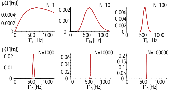
Figure 31: Probability distributions for a sequence of tunneling times \{\tau_i\} to belong to a physical process being characterized by the tunnel coupling \Gamma . The different graphs correspond to different lengths of the data set.
