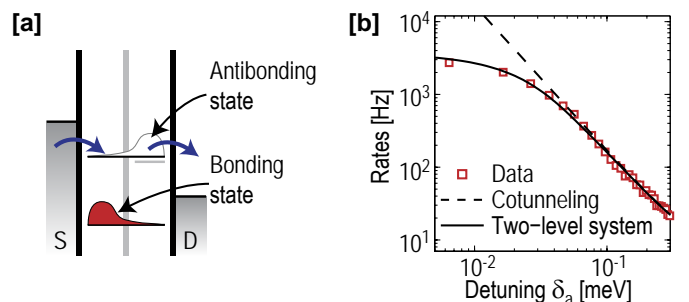
Figure 40: (a) Cotunneling described using molecular states. Due to the large detuning the empty antibonding state is mainly localized on QD2, but a small part of the wavefunction is still present in QD1 which allows an electron to enter from the source. (b) The rate for electrons tunneling into the DQD ( \Gamma_{\text{in}} ) as a function of DQD detuning \delta_a . The figure shows the same data as in Fig. 39, but plotted on a log-log scale to enhance the features at small detuning. The dashed line is the results of the cotunneling model in Eq. (74), the solid line shows the result of the molecular-state model [Eq. (75)]. Adapted from Ref. [66].
