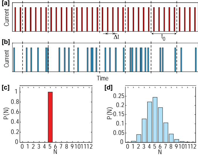
Figure 17: (a) Idealized current flow. Each spike corresponds to an electron passing the conductor, with constant time intervals between electrons. (b) Same as (a), but for a realistic current. The electron flow shows random variations. (c-d) Distribution function for the currents shown in (a-b). The distribution function is formed by counting the number of electrons passing the conductor within a time t_0 .
