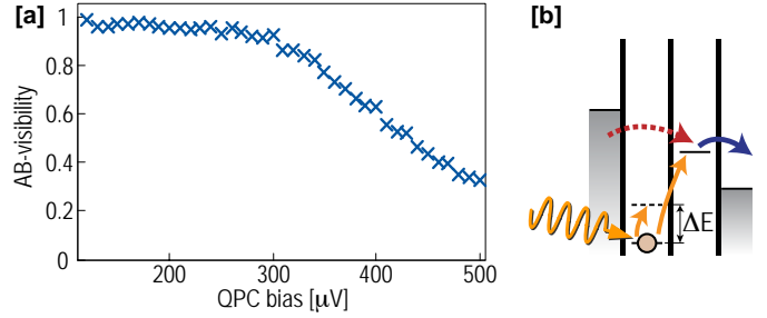
Figure 65: (a) Visibility of the AB-oscillations measured at different QPC bias. The visibility stays roughly constant up to V_{QPC} = 300 \mu\text{V} and then decreases drastically with increasing bias voltage. We attribute the reduction in visibility to an increase in photon-assisted tunneling. (b) Energy level diagram of the DQD in the cotunneling configuration. At high QPC bias, both intradot and interdot photon absorption processes become possible. Adapted from Ref. [69].
