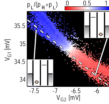
Figure 54: Average population of state L , measured for the same region as shown in Fig. 52(a). The insets show the DQD level configurations for positive and negative detuning, the dashed line defines the detuning axis.
