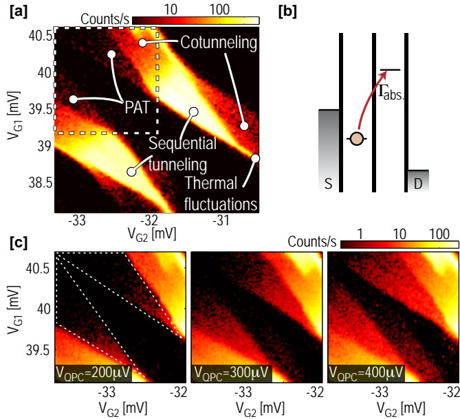
Figure 57: (a) Charge stability diagram for the DQD, measured with a bias voltage V_{\text{DQD-SD}} = 300 \mu\text{V} applied over the DQD. Tunneling due thermal fluctuations, sequential transport, cotunneling and photon-assisted processes (PAT) are visible. The data was taken with V_{\text{QPC-SD}} = 300 \mu\text{V} . (b) DQD energy level diagram for the upper region of photon-assisted tunneling in (a). The detuning is opposite to the bias direction. (c) Magnifications of the region marked by the dashed rectangle in (a), measured for three different QPC bias voltages. The dashed lines in the leftmost figure show the regions where we expect photon-assisted tunneling. As the QPC bias voltage is increased, the count rate goes up inside the PAT regions.
