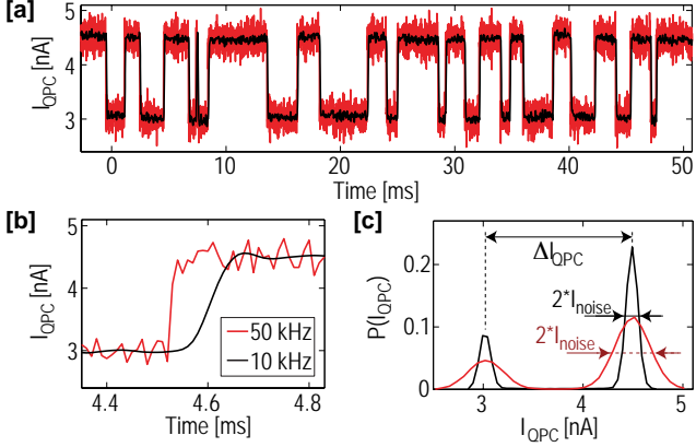
Figure 4: (a) Time trace of the current through the quantum point contact, showing a few transitions due to electrons tunneling into and out of the QD. The two traces are taken with 10 kHz and 50 kHz bandwidth. (b) Blow-up of one switching event from the trace in (a). The rise time is clearly different for the data taken with 10 kHz and 50 kHz bandwidth. (c) Histogram showing the distribution of the current for the data in (a). The two levels are easily distinguished.
