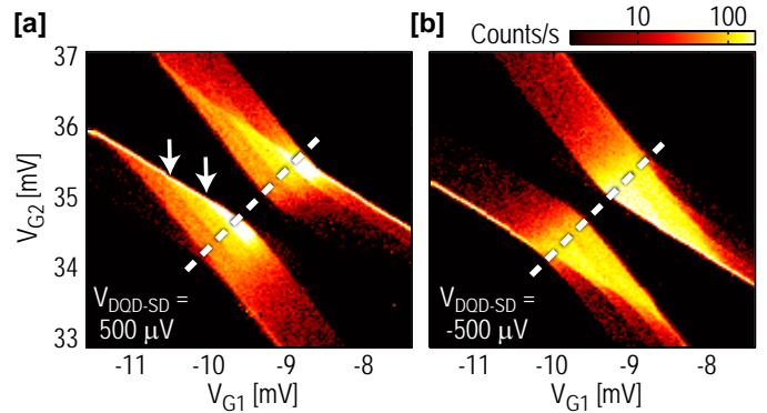
Figure 41: Finite-bias spectroscopy of the DQD, taken with positive (a) and negative (b) bias. The figures are constructed by counting electrons entering and leaving the DQD. Excited states are visible, especially for the positive bias data [marked with arrows in (a)]. The data was taken with V_{\text{DQD-SD}} = \pm 500 \mu\text{V} , V_{\text{QPC-SD}} = 250 \mu\text{V} . Adapted from Ref. [66].
