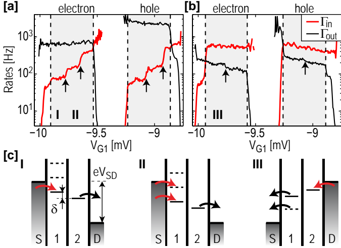
Figure 42: (a, b) Tunneling rates for electrons entering and leaving the DQD, measured along the dashed lines in Fig. 41(a, b). In (a), we show the results for positive bias across the DQD, in (b) the results for negative bias. The shaded areas mark the regions where electron transport is sequential, either in the electron or the hole transport cycle. The arrows indicate the positions of excited states. The data was extracted from QPC conductance traces of length T = 5 s, taken with V_{QPC-SD} = 250 mV. (c) Schematics of the DQD energy configuration at three different positions in (a, b). Adapted from Ref. [66].
