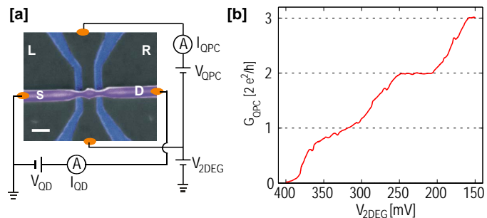
Figure 1: (a) Quantum point contact, defined by etching trenches (marked in blue in the figure) in a GaAs heterostructure containing a 2DEG 37 nm below the surface. A quantum dot defined in an InAs nanowire (purple) is lying on top of the structure. (b) Conductance of the QPC versus voltage applied to the 2DEG. The measurement was performed in a two-terminal setup, with V_{\text{QPC-SD}} = 200 \mu\text{V} applied across the QPC. A series resistance of 4 \text{ k}\Omega was subtracted because of the ohmic contact resistance. The measurement was performed at a temperature of T = 1.7 \text{ K} .
