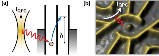
Figure 51: Schematic for operating a double quantum dot (DQD) as a high-frequency noise detector. The tunable level separation \delta of the DQD allows frequency-selective detection. (b) The double quantum dot used in the experiment.
