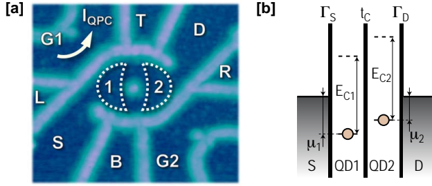
Figure 33: (a) AFM-image of the sample investigated in this section. The structure consists of a double quantum dot (DQD) (marked by 1 and 2) with a nearby quantum point contact. (b) Energy level diagram of the DQD. The QDs are tunnel coupled to source and drain leads with tunneling rates \Gamma_S and \Gamma_D , while the interdot transitions are characterized by the coupling energy t_C .
