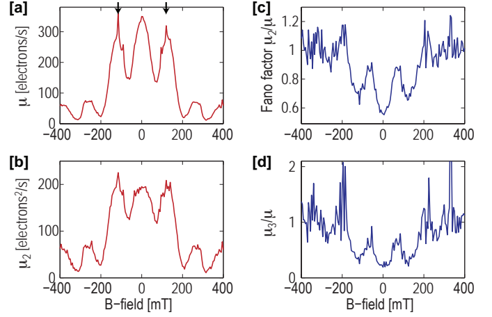
Figure 62: (a) DQD current in the Aharonov-Bohm regime. (b) Noise \mu_2 of the DQD current. The curve strongly resembles the average current shown in (a), with the AB-oscillations clearly visible. (c-d) Fano factor \mu_2/\mu and generalized Fano factor for the third moment ( \mu_3/\mu ), measured within the same region as the traces shown in (a, b). All quantities were extracted from a QPC conductance traces of length T = 40 s, measured with V_{DQD-SD} = 600 \mu V and V_{QPC-SD} = 300 \mu V .
