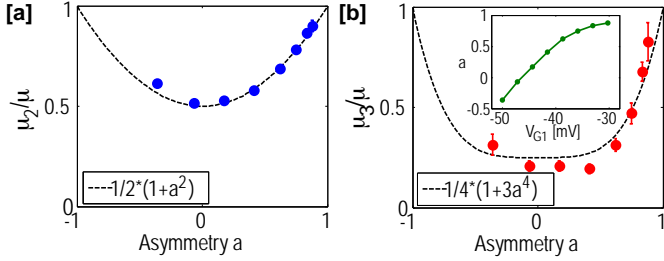
Figure 22: (a) Second and (b) third normalized central moments of the fluctuations of n as a function of the asymmetry of the tunneling rates, a = (\Gamma_{\text{in}} - \Gamma_{\text{out}})/(\Gamma_{\text{in}} + \Gamma_{\text{out}}) . To increase the resolution, each point at a given asymmetry is obtained by averaging over about 50 points at a given voltage V_{G1} and in a window of bias voltage 1.5 < V_{\text{SD}} < 3 mV. Error bars correspond to the standard error of this averaging process, and are of the size of the points if not shown. The dashed lines are the theoretical predictions given by Eqs. (39, 41). No fitting parameters have been used, since the tunneling rates are fully determined experimentally. Inset of (b): Variation of the asymmetry of the tunneling rates, a , as a function of V_{G1} . Adapted from Ref. [40].
