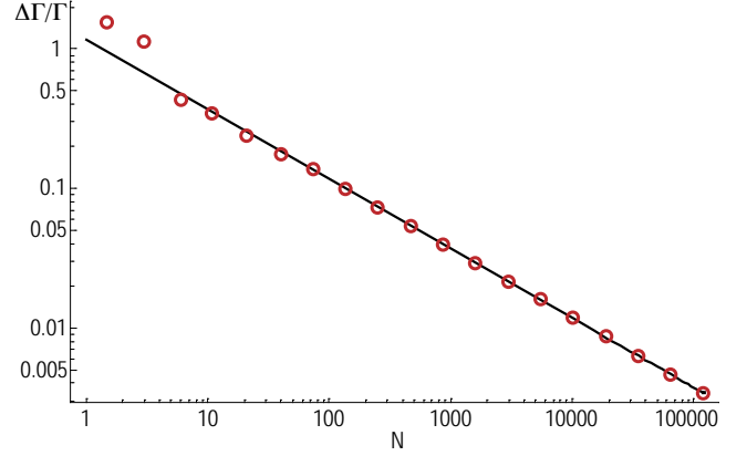
Figure 32: Accuracy achieved when determining the tunnel coupling \Gamma versus the size of the data set. The accuracy was measured by taking the width of the distributions as shown in Fig. 31. The solid line is the result of Eq. (66)
