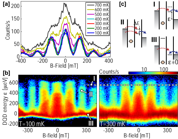
Figure 63: (a) Aharonov-Bohm (AB) oscillations measured at different temperatures. At \sim 400 mK, the visibility of the oscillations drops drastically. The data was taken along the dashed line in (b). (b) Rate of electrons entering QD2, measured versus B-field and total energy of the DQD, \varepsilon . The two images show data taken at two different temperatures, T = 100 mK and T = 300 mK. The DQD energy \varepsilon is taken to be zero when QD2 is aligned with Fermi level of the drain. Here, tunneling due to thermal fluctuations between QD2 and the lead gives rise to a high count rate (point III). This feature is visibly broadened when the temperature is increased. In the cotunneling region (point I), the count rate shows clear AB oscillations. The elevated temperature only has a slight impact on the AB-visibility. In case II, the cotunneling rate goes up compared to case I. We attribute the increase to tunneling into an excited state in QD2. (c) Diagrams depicting DQD energy levels for the three configurations marked in (b).
