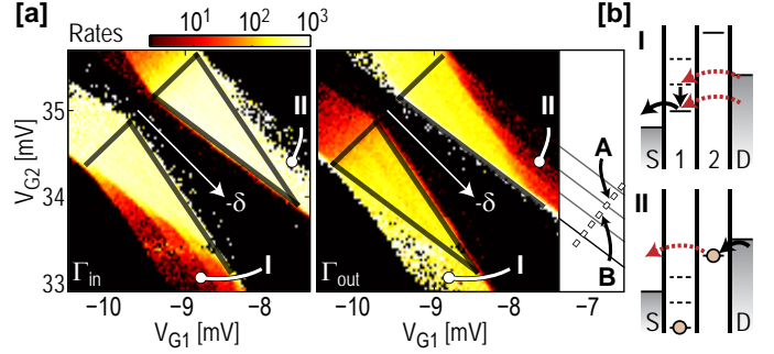
Figure 43: (a) Tunneling rates for electrons entering and leaving the DQD, extracted from the same set of data as used in Fig. 41(b). The data was measured with V_{DQD-SD} = -500 \mu\text{V} . The solid lines mark the position of the finite-bias triangles. The plot region in the right-hand panel has been extended to include the regime investigated in Fig. 44. (b) Energy-level diagrams for the two positions marked in (a). In case I, the cotunneling itself is elastic, with energy relaxation occurring after the cotunneling has taken place. In case II, inelastic cotunneling processes are possible. Adapted from Ref. [66].
