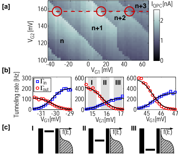
Figure 15: (a) Current through the QPC as a function of voltage on gates G_1 , G_2 . The diagonal lines show positions where the population of the QD changes by one electron. The numbers specify the dot occupation in the different regions. (b) Effective tunneling rates for electrons entering and leaving the dot, measured at the three charge degeneracy points marked by circles along the dashed line in (a). The solid lines are fits using Eqs. (25, 26), with T = 230 mK and the other fitting parameters given in Table 1 in the text. (c) Alignment of the QD electrochemical potential relative to the Fermi level of the lead for the gate voltage configurations shown in the middle plot in (b). Adapted from Ref. [30].
