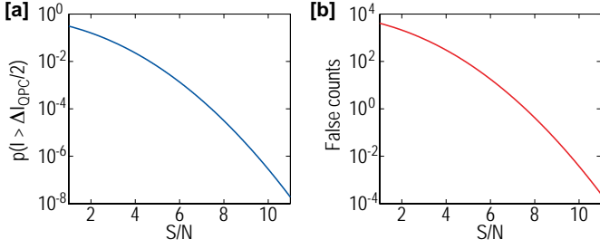
Figure 5: (a) Part of the QPC current having I > \Delta I_{\text{QPC}}/2 , assuming a Gaussian distribution. (b) Average number of false counts, calculated from Eq. (5) in the text with \Delta t = 1 s and f_{\text{BW}} = 10 kHz. The risk of detecting false events falls off rapidly with increased S/N.
