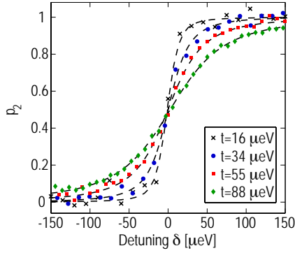
Figure 38: Charge population on QD2, evaluated from the change in QPC current \Delta I_{\text{QPC}} for one electron entering the DQD. The different traces were taken at different gate voltages. The dashed lines are fits to Eq. (73), with T = 100 mK.
