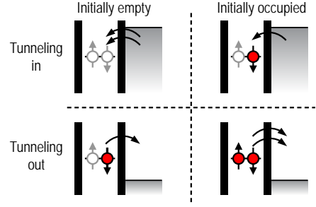
Figure 16: Effective tunneling rates for spin degenerate states in different configurations. The empty circles represent empty spin states, filled circles represent occupied ones. The arrows depict the number of possible tunnel processes.
