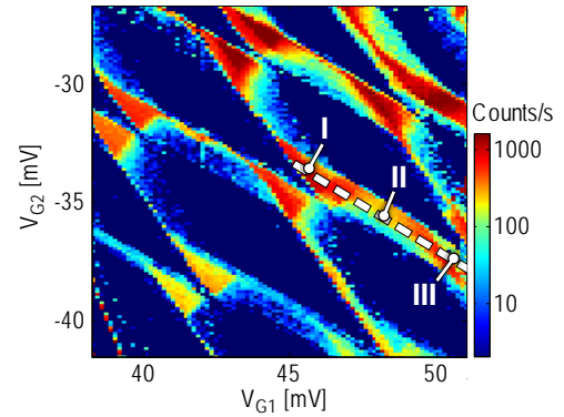
Figure 59: Charge stability diagram of the double quantum dot, recorded by counting electrons entering and leaving the structure. The data was taken at DQD bias voltage V_{\text{DQD-SD}} = 600 \mu\text{V} and B = 0 \text{ T} . The dashed line marks the region of cotunneling used for measuring single-electron Aharonov-Bohm interference.
