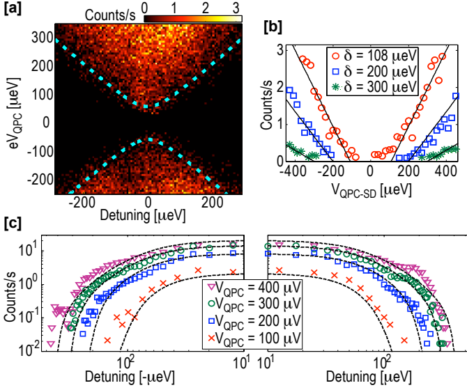
Figure 55: Count rate measured versus detuning and QPC bias voltage. The dashed line shows the level separation for a two-level system, with \Delta_{12} = \sqrt{4t^2 + \delta^2} . There are only counts in the region where |eV_{\text{QPC}}| > \Delta_{12} . (b) Count rate versus QPC bias for different values of detuning. The solid lines are guides to the eye. (c) DQD absorption spectrum, measured for different QPC bias. The dashed lines are the results of Eq. (85), with parameters given in the text. Adapted from Ref. [12].
