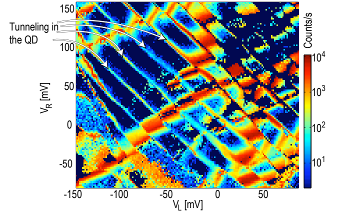
Figure 8: Same as Fig. 7, this time measured for a QPC defined by etching. The switches due to traps are more frequent than in the AFM-defined sample, possibly because of surface states formed in the etched trenches. The data was also taken at a higher electron temperature ( T = 1.7 \text{ K} instead of 200 mK)
