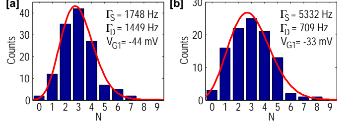
Figure 19: Statistical distribution of the number N of electrons entering the QD during a given time t_0 . The two panels correspond to two different values of the tunneling rates, obtained for different values of the gate voltage V_{G1} . The time t_0 is chosen in order to have the same mean value of number of events, \langle N \rangle \approx 3 , for both graphs. The line shows the theoretical distribution calculated from Eqs. (36) and (35). The tunneling rates are determined experimentally by the method described in Chapter 2, and no fitting parameters are involved in the curves showing theoretical results. Adapted from Ref. [40].
