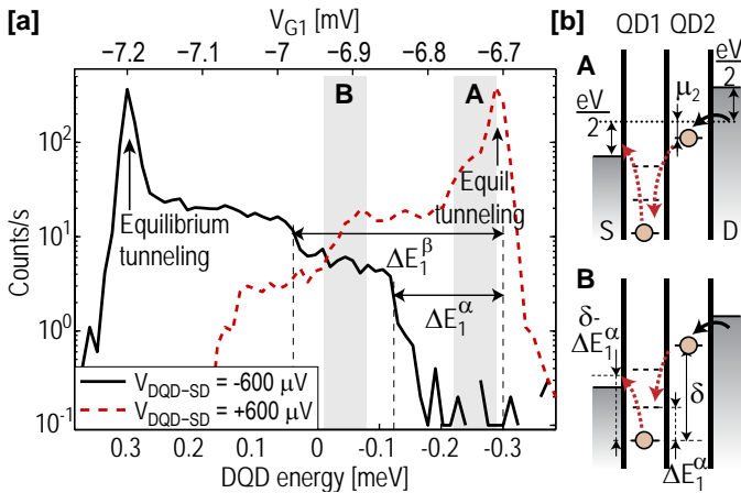
Figure 44: (a) Electron count rate along the dashed line in Fig. 43(a), measured for both positive and negative DQD bias. In the trace, the detuning \delta stays constant and we sweep the average DQD energy. The DQD energy is defined from the position where the electrochemical potential of QD2 is right in the middle between the Fermi levels of the source and drain leads [see the dotted line in the energy level diagram in (b)]. The steps in the count rate are due to the onset of inelastic cotunneling processes in QD1. The data was extracted from traces of length T = 10 s, measured with V_{QPC-SD} = 200 \mu\text{V} . (b) Energy level diagrams for the two configurations marked in (a). Adapted from Ref. [66].
