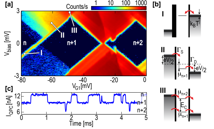
Figure 12: (a) Coulomb diamonds, measured by counting electrons entering the QD. For low values of V_{G1} , the source lead is pinched off and tunneling can only occur between the dot and the drain lead. As V_{G1} increases, the source lead opens up and a current can flow through the dot. (b) Diagrams depicting the energy levels of the dot at points I, II and III. In case III, the bias is higher than the charging energy of the dot, meaning that the dot may hold 0, 1 or 2 excess electrons. (c) Time trace taken at point III. The three possible dot population ( n , n + 1 or n + 2 electrons) are clearly resolvable. Adapted from Ref. [20].
