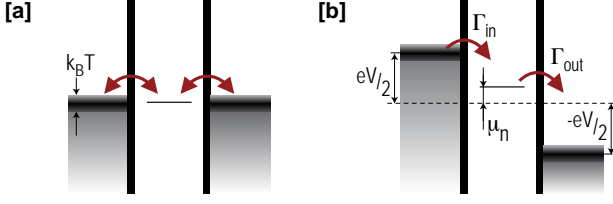
Figure 18: (a) Energy level diagram for the quantum dot in the regime of equilibrium fluctuations. Electrons may leave or enter the dot from either of the two leads. (b) Energy level diagram for the quantum dot in the high bias regime. With a large bias applied to the QD, and with the Fermi levels of the leads far away from the electrochemical potential of the dot, electrons can only enter the QD from the source lead and only leave to the drain.
