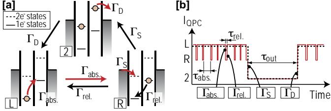
Figure 53: (a) Energy level diagrams for the three states of the DQD. The labels L , R and 2 denote the excess charge population. The levels are raised by the intradot charging energy E_{Ci} when the DQD holds two excess electrons. (b) Schematic changes of the detector signal as electrons tunnel into, between and out of the DQD. Adapted from Ref. [12].
