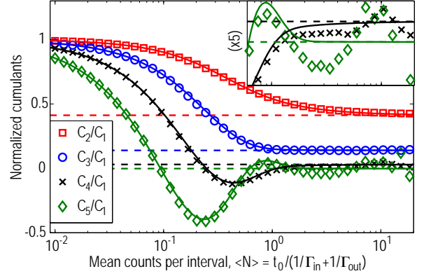
Figure 30: Normalized cumulants evaluated for different lengths of the time interval t_0 . The symbols show the experimental data, extracted from a time trace of length T = 10 minutes, containing 350595 events, with a = 0.053 , and \Gamma_{\text{tot}} = 3062 Hz. The solid lines are calculations from the FCS given by Eq. (53) in the text, while the dashed lines are the asymptotes for t_0 \rightarrow \infty . The inset shows a magnification of the vertical axis (horizontal axis unchanged) for C_4/C_1 and C_5/C_1 for \langle N \rangle > 0.6 . Adapted from Ref. [60].
