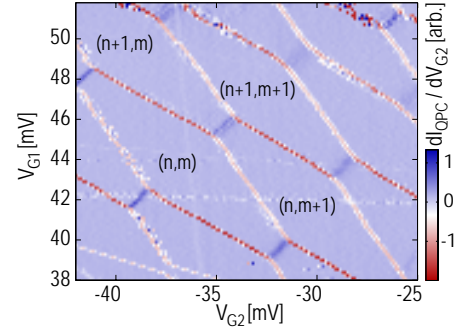
Figure 34: Numerical derivative of the QPC current with respect to the voltage on gate G2. A positive derivative reflects an increase in QPC conductance, which means that an electron is moving away from the QPC. For a negative derivative, an electron is coming closer to the QPC. The horizontal white line most likely originates from electron fluctuations of a charge trap. The numbers in the figure refer to the number of electrons in the two QDs. The data was taken with QPC bias V_{\text{QPC-SD}} = 400 \mu\text{V} and zero bias across the DQD.
