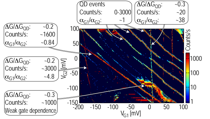
Figure 7: Count rates for a single QD, measured vs voltage on the two gates G1 and G2. Apart from the transitions due to electrons tunneling into and out of the QD, there are several other lines present in the figure. These originate from charge traps sitting in the substrate close to the QPC. Such events can be distinguished from tunneling in the QD by investigating the change of the QPC conductance or looking at how the switches depend on gate voltages. The boxes describe some of the transitions, where \alpha_{G1/G2} is the capacitive lever arms of the gates relative to the trap. The electron temperature was 200 mK.
