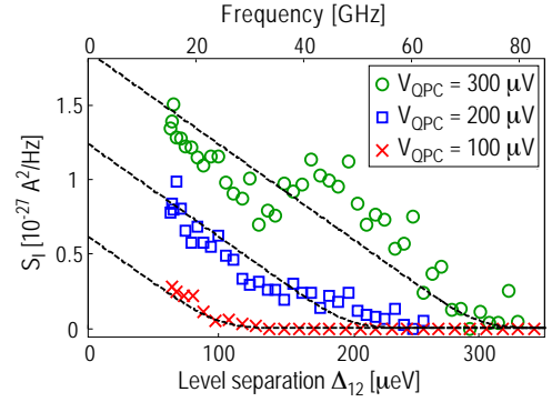
Figure 56: Noise spectrum of the QPC, extracted from the data in Fig. 55(c). The dashed lines show spectra expected from Eq. (84). Adapted from Ref. [12].
