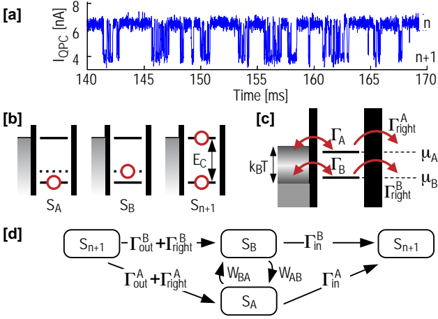
Figure 24: (a) Time trace of the QPC current showing bunching of electrons. (b) Dot states included in the model used to describe the bunching of electrons. The red circles correspond to electron occupation. State S_A is the n -electron ground state, state S_B is an excited n -electron state and state S_{n+1} is the ground state when the dot contains (n+1) electrons. (c) Energy diagram for the model. The two dot transitions are both within the thermal broadening of the lead. Electrons enter the dot from the left lead and may leave through either the left or the right lead. (d) Possible transitions between the different states of the model. The rates \Gamma_{\text{in}}^A, \Gamma_{\text{in}}^B refer to electrons entering the QD from the left lead, thus taking the dot from state S_{A/B} to state S_{n+1} . The rates \Gamma_{\text{out}}^A, \Gamma_{\text{out}}^B describe electrons leaving the dot to the left lead, giving transitions from state S_{n+1} to S_{A/B} . W_{AB} and W_{BA} are the direct transition rates between states S_A and S_B . Finally, the rates \Gamma_{\text{right}}^A, \Gamma_{\text{right}}^B refer to electrons leaving the dot through the right lead. Adapted from Ref. [20].
