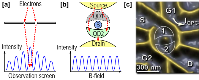
Figure 58: (a) Setup of a traditional double-slit experiment. Electrons passing through the two slits give rise to an interference pattern on the observation screen. (b) Schematic drawing of the setup used for measuring single-electron Aharonov-Bohm interference. Electrons are injected from the source lead, tunnel through QD1 and end up in QD2, where they are detected. The interference pattern is due to the applied B-field, which introduces a phase difference between the left and right arm connecting the two quantum dots. (c) Double quantum dot used in the experiment. The yellow parts are lines written with a scanning force microscope on top of a semiconductor heterostructure and represent the potential landscape for the electrons. The QDs (marked by 1 and 2) are connected by two separate arms, allowing partial waves taking different paths to interfere. The current in the nearby QPC ( I_{\text{QPC}} ) is used to monitor the electron population in the system. Adapted from Ref. [69].
