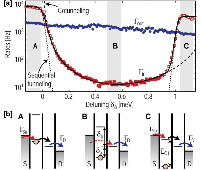
Figure 39: Tunneling rates for electrons entering and leaving the DQD, measured while keeping the potential of QD2 fixed and sweeping the electrochemical potential of QD1. The data is measured in a configuration similar to going along the dashed line in Fig. 35(a). The dotted lines are tunneling rates expected from sequential tunneling, while the dashed line is a fit to the cotunneling model of Eq. (74). The solid line corresponds to the model involving molecular states [Eq. (75)]. Parameters are given in the text. (b) Schematic drawings of the DQD energy levels for three different configurations in (a). At point A, electrons tunnel sequentially through the structure. Moving to point B, the energy levels of QD1 are shifted and the electron in QD1 is trapped due to Coulomb blockade. Electron transport from source to QD2 is still possible through virtual processes, but the rate for electrons entering the DQD drops substantially due to the low probability of the virtual processes. At point C, the next level of QD1 is brought inside the bias window and sequential transport is again possible. Adapted from Ref. [66].
