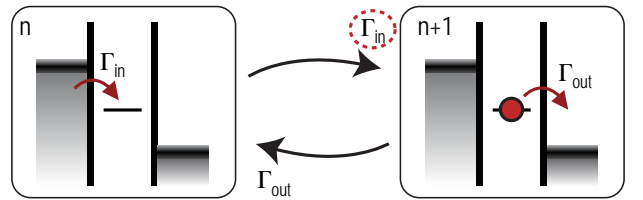
Figure 20: State diagram of a two-state model describing electron tunneling in a QD in the single-level regime. Transitions between the states occur with rates \Gamma_{\text{in}} and \Gamma_{\text{out}} . The counting field e^{i\chi} is introduced for the transition involving an electron entering the QD, as marked by the dashed circle.
