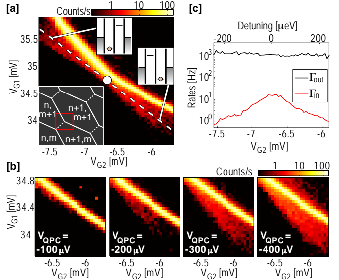
Figure 52: (a) Count rate for electrons leaving the DQD, measured for a small region close to a triple point (marked by a white point). The inset shows a sketch of the surrounding hexagon pattern. The dashed line denotes the detuning axis, with zero detuning occurring at the triple point. The data was taken with V_{\text{QPC}} = -300 \mu\text{V} . (b) Blow-up of the lower-right region of (a), measured for different QPC bias voltages. (c) Rates for electron tunneling into and out of the DQD, measured along the dashed line in (a). \Gamma_{\text{in}} falls off rapidly with detuning, while \Gamma_{\text{out}} shows only minor variations. Adapted from Ref. [12].
