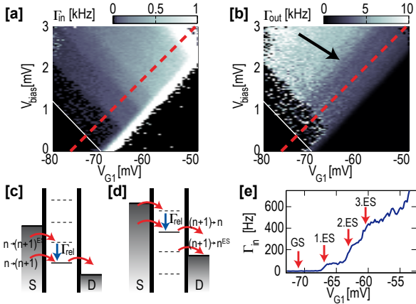
Figure 13: (a) and (b): Blow-up of the upper left region of Fig. 12(a), showing the rates for electrons tunneling into (a) and out of (b) the QD, respectively. The white solid lines mark the positions where the source lead lines up with the electrochemical potential of the QD ground state. The dashed lines mark the lower edge of the region where condition of Eq. (18) in the text is fulfilled. The color scales are different for the two figures, the rate for tunneling out is roughly 10 times faster than tunneling in. (c) Diagram depicting the energy levels along the dashed lines in (a) and (b). As the source lead is raised [corresponds to going upward along the dashed lines in (a)], excited states become available for tunneling. (d) Energy diagram for the configuration marked by the arrow in (b). Here, the excited states is visible in the rate for electrons tunneling out of the QD. (e) Tunneling rate for electrons entering the dot, measured along the dashed line in (a). Three excited states are clearly resolvable. Adapted from Ref. [20].
