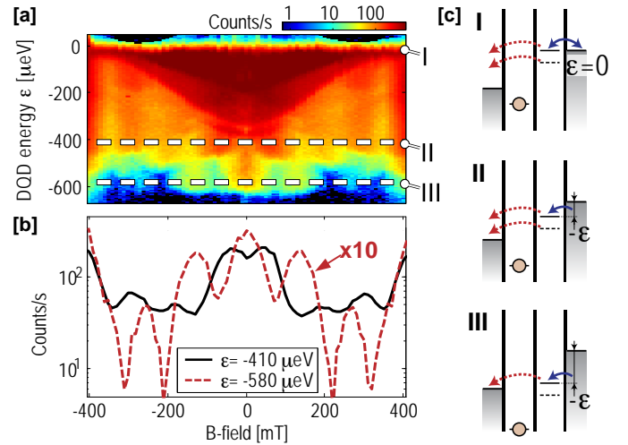
Figure 64: (a) Electron count rate, measured versus magnetic field and total DQD energy relative to the leads, \varepsilon . The data was measured with V_{\text{DQD-SD}} = -600 \mu\text{V} applied to the DQD. (b) Count rates measured at the positions marked by the dashed lines in (a). There is a phase shift of \sim 0.7\pi between the two curves. The trace for \varepsilon = -580 \mu\text{eV} has been magnified by a factor of ten for better visibility. (c) Energy diagrams of the DQD for the positions marked by I, II and III in (a). At point I, the potential of QD2 is lined up with the Fermi level in the right lead and the tunneling is mainly due to equilibrium fluctuations between QD2 and the lead. At point II, the DQD potential is shifted downwards, so that electrons in QD2 may only leave by cotunneling to the source lead. The energy level arrangement allows a process involving an excited states of QD2 to contribute to the cotunneling. Finally, at point III only cotunneling involving the ground state of QD2 is possible. Adapted from Ref. [116].
