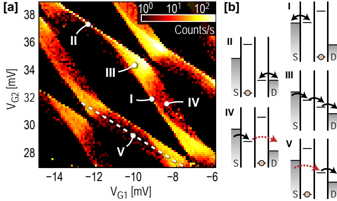
Figure 35: (a) Charge stability diagram of the DQD, measured by counting electrons entering and leaving the DQD. The data was taken with a voltage bias of V_{\text{DQD-SD}} = 600 \mu\text{V} applied over the DQD. The QPC conductance was measured with V_{\text{QPC-SD}} = 300 \mu\text{V} . The count rates were extracted from traces of length T = 0.5 \text{ s} . (b) Energy level diagrams for different configurations in (a). Adapted from Ref. [66].
