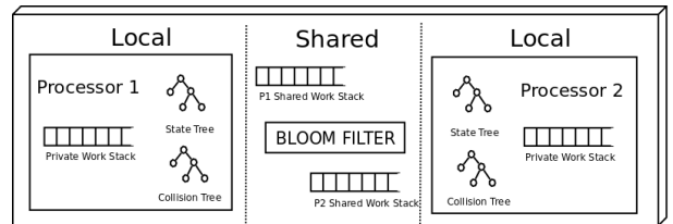
Figure 2. Shared and Private Data Model Scheme.
