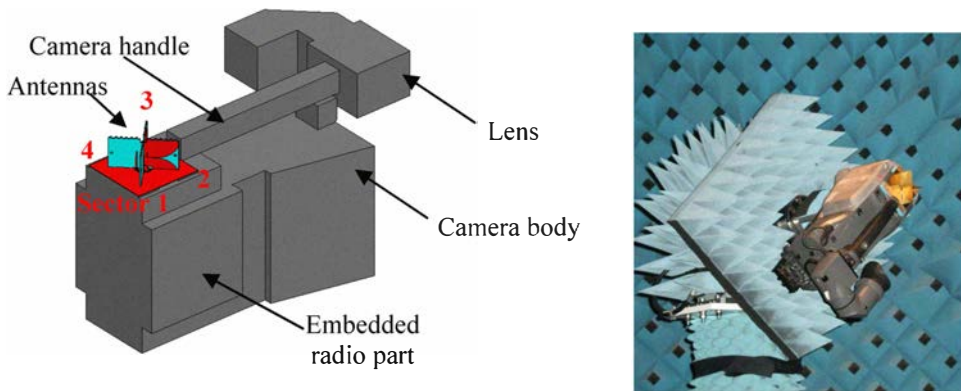
Figure 2: Camera + antenna system global views.
