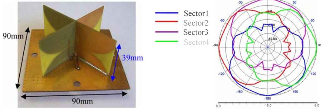
Figure 1: 4-sector switched beam antenna in FR4 substrate and associated radiation pattern at 6GHz in the azimuth plane ( \theta=90^\circ ).
