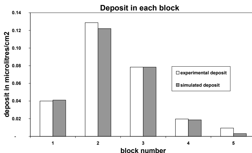
Figure 5. Comparison between experimental and simulated deposit.
