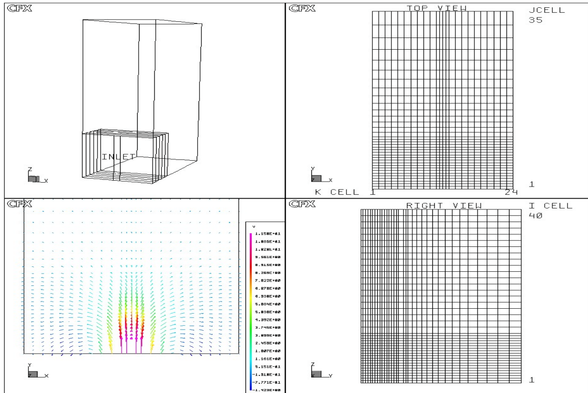
Figure 2. Geometry. Top left, global geometry. Top right, grid from top view. Bottom right, grid from right view. Bottom left, simulation air flow.
