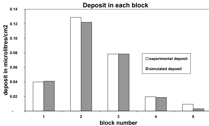
Figure 5. Comparison between experimental and simulated deposit.
