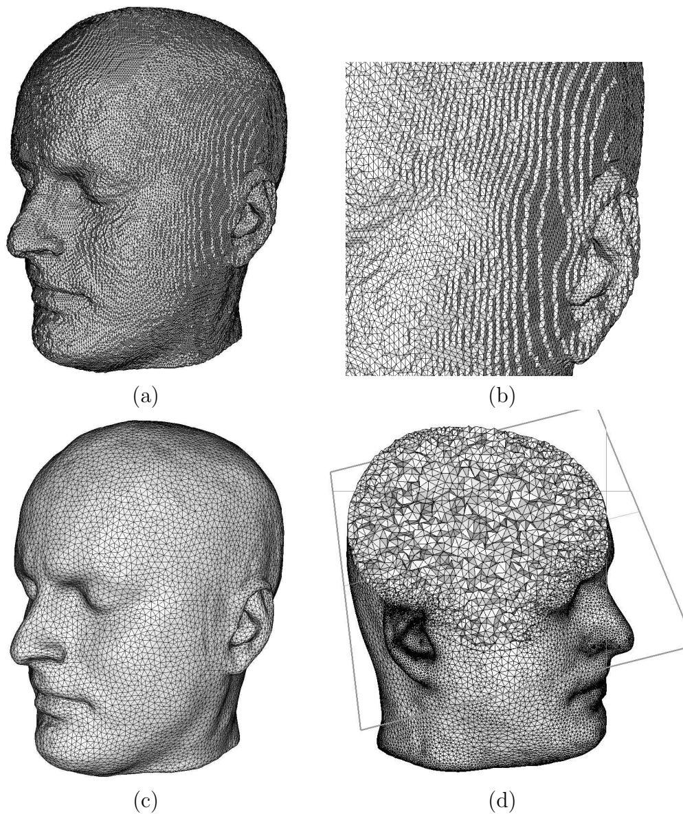
Figure 5: (a,b) Surface triangulation obtained from MRI slices , (c) Surface triangulation adapted to the geometric properties , (d) Generation of a three-dimensional triangulation .
