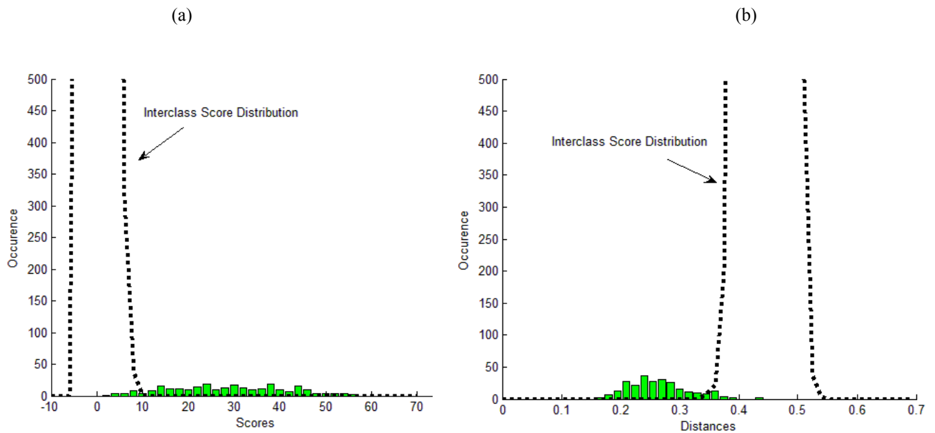
Fig.10 Intraclass score distribution for CORR system on Fig. 10(a) and for OSIRIS system on Figure 10(b) when comparing good quality reference images with rotated test images (256 comparisons). The interclass score distribution in each case is represented by a dashed line curve after zooming for a better view.
