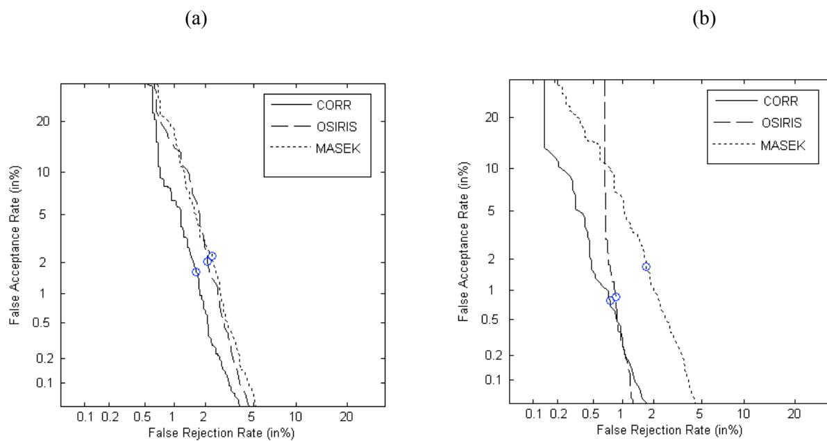
Fig.6 DET curves of CORR system (solid curve), OSIRIS system (dashed curve) and MASEK (dotted curve) on: (a) Bad and average quality subset (quality 3: 18 images and quality 4: 392 images), (b) Good quality subset (quality 5: 1015 images), of
