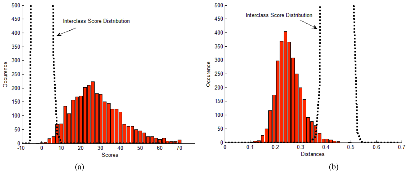
Fig.9 Intraclass score distribution for CORR system on Fig. 9(a) and for OSIRIS system on Figure 9(b) when comparing good quality reference images with blurred test images (3035 comparisons). The interclass score distribution in each case is represented by a dashed line curve after zooming for a better view.
