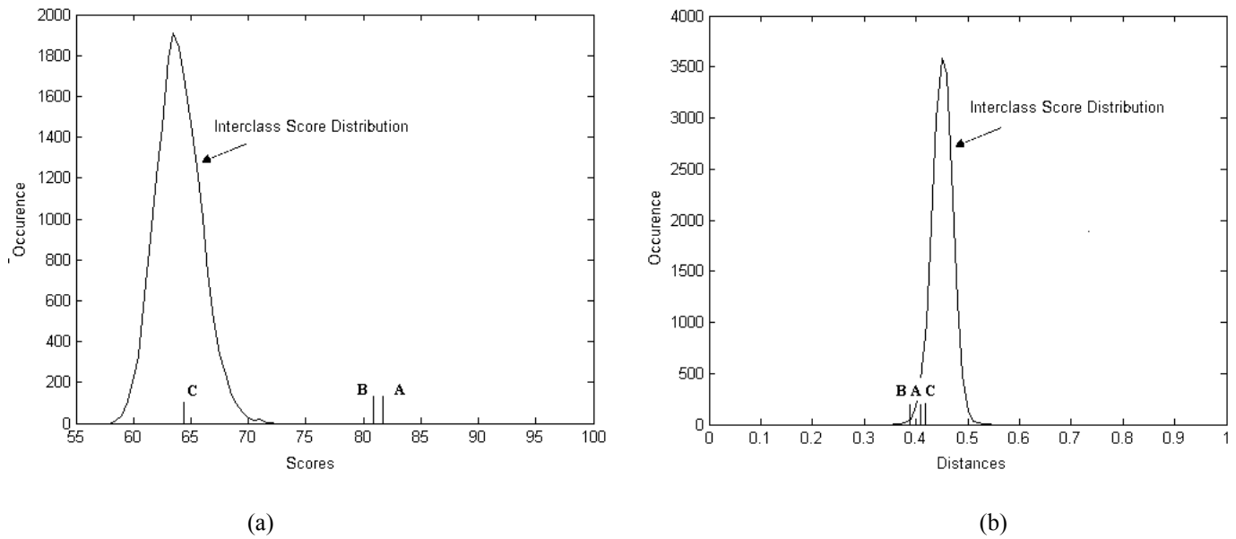
Fig.8 Results of 3 challenging intraclass image comparisons (shown in Figure 7): mark A stands for comparison of images 7(d) v.s. 7(e), mark B stands for comparison of images 7(e) v.s. 7(b) and mark C stands for comparison of images 7(f) v.s. 7(c). Figure 8(a) shows results for CORR system and Figure 8(b) shows results for OSIRIS system.
