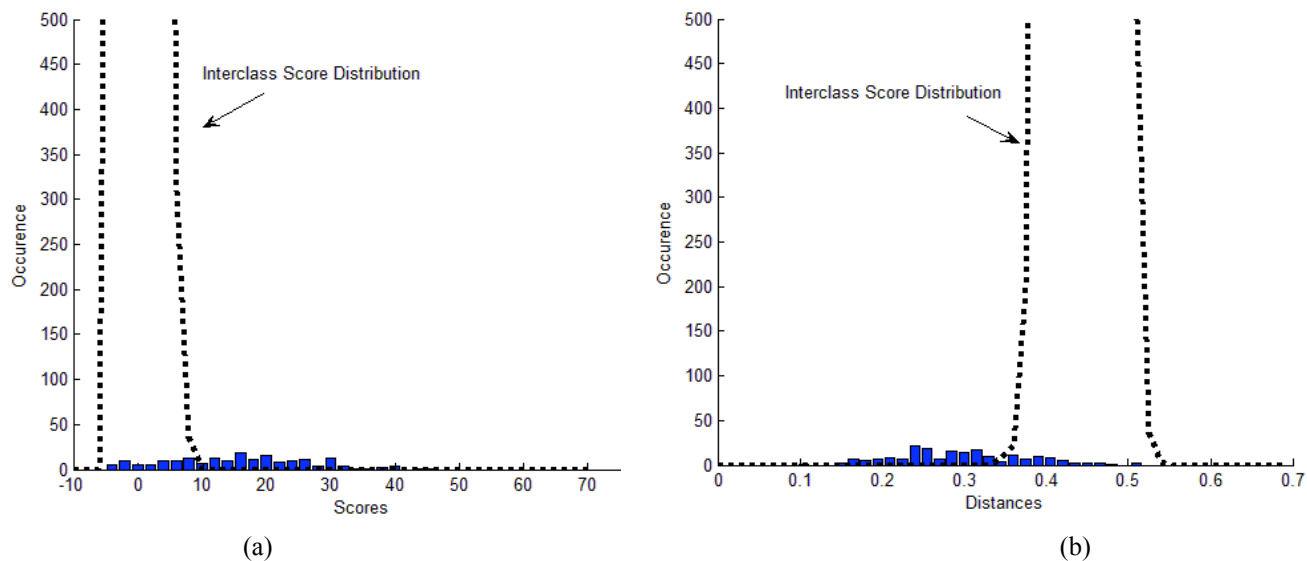
Fig.11 Intraclass score distribution for CORR system on Fig. 11(a) and for OSIRIS system on Figure 11(b) when comparing good quality reference images with occluded test images (189 comparisons). The interclass score distribution in each case is represented by a dashed line curve after zooming for a better view.
