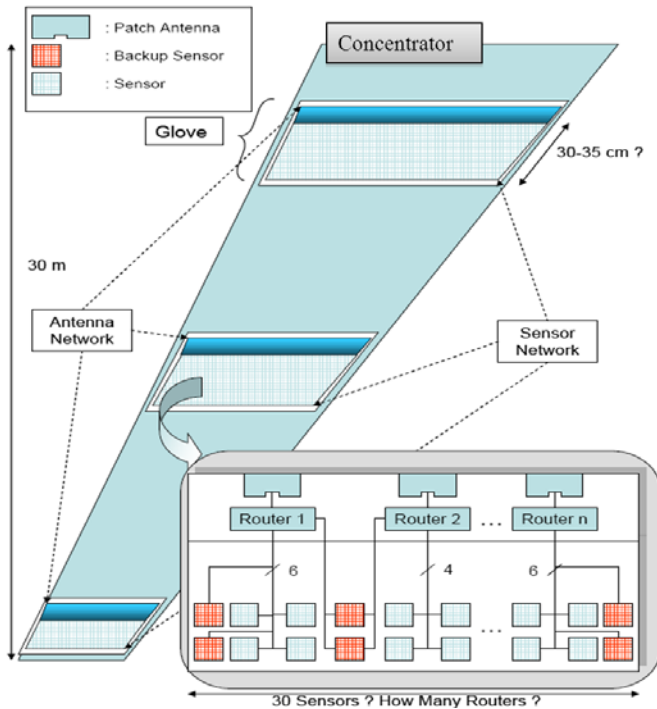
Figure 1: Wireless Sensor Network Architecture in the aircraft wings
