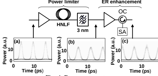
Fig. 4. Regenerator setup.
