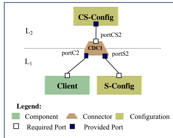
b: Possible links of CDC1 connector
