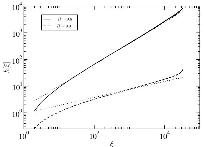
Figure 3: Ordered and averaged sequence \bar{h}[\xi] based on 1000 self-affine h(x) with Hurst exponents equal to 0.8 and 0.3 respectively. The data consists of 1000 samples of length 2^{15} . The straight lines are \xi^{0.8} and \xi^{0.3} respectively.
