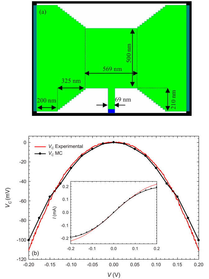
FIG. 6. (Color online) (a) Geometry of the MC simulation domain for the TBJ with W_H=500 nm. (b) Comparison of measured and simulated values of V_C vs push-pull bias V for the TBJ with W_H=500 nm. Inset: I - V curve obtained using a nonsimulated dimension Z=10^{-7} m.
