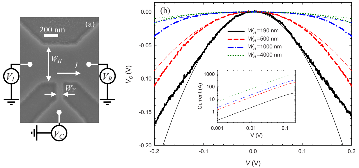
FIG. 1. (Color online) (a) SEM image of one of the fabricated TBJs. (b) Values of the bottom potential V_C and current I (inset) measured in TBJ junctions with W_H=190, 500, 1000, and 4000 nm as a function of the push-pull bias V . The width of the vertical branch W_V is approximately the same, 70 nm. Hair lines show parabolic fittings.
