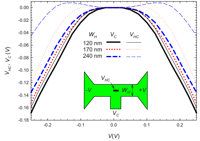
FIG. 4. (Color online) V_{HC} - V and V_C - V curves as obtained from MC simulations for TBJs with W_H = 120, 170, and 240 nm. The width of the vertical branch W_V is 108 nm.
