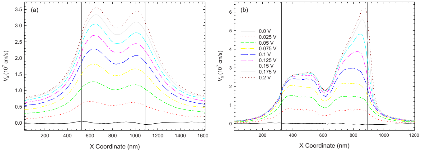
FIG. 7. (Color online) Profiles of longitudinal velocity along the horizontal branch for push-pull bias voltages between 0.0 and 0.2 V in TBJs with (a) W_H = 500 nm and (b) W_H = 120 nm. Vertical lines delimit the active region of each TBJ.
