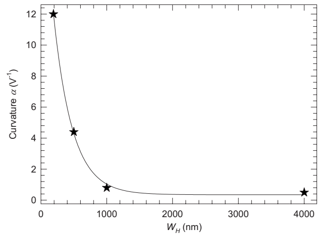
FIG. 2. Curvature factor \alpha as a function of the width of the horizontal branch W_H . The continuous line shows the fitting according to Eq. (1).
