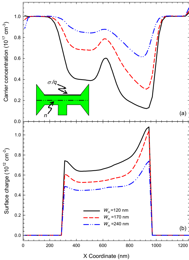
FIG. 5. (Color online) Profiles of (a) carrier concentration, n , along the horizontal direction (left axis) and (b) surface charge, \sigma/q , at the top boundary of the junction (right axis) in TBJs with W_H=120 , 170, and 240 nm for a push-pull bias V=0.25 V.
