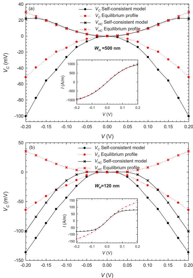
FIG. 8. (Color online) MC results for V_C - V and V_{HC} - V curves in TBJs with (a) W_H = 500 nm and (b) W_H = 120 nm simulated with the self-consistent surface charge model and also with the surface charge fixed to the equilibrium profile. Insets: current flowing through the horizontal branch.
