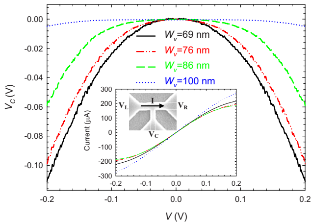
FIG. 3. (Color online) Values of the bottom potential V_C and current I (inset) measured in TBJ junctions with a width of the vertical branch W_V of 69, 76, 86, and 100 nm as a function of the push-pull bias V . W_H = 500 nm.
