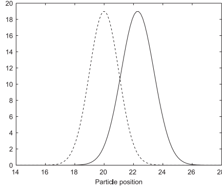
FIGURE 2. Plot of the first-stage importance weight functions t_4^* (unbroken line) and t_4^{\text{P\&S}} (dashed line) in the presence of an outlier
