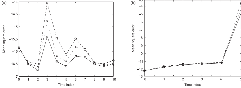
FIGURE 1. Plot of MSE performances (on log-scale) of the bootstrap particle filter (*), the SSAPF based on optimal weights ( \square ), and the SSAPF based on the generic weights t_k^{\text{P\&S}} of Pitt and Shephard [17] ( \circ ). The MSE values are founded on 100,000 particles and 400 runs of each algorithm
