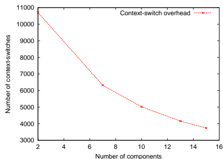
Fig. 12: The REMORA-based implementation does not impose additional CPU overhead compared to the Contiki-based implementation. Fig. 13: As the number of producer components in the queue is increased, the number of context switches is significantly decreased.
