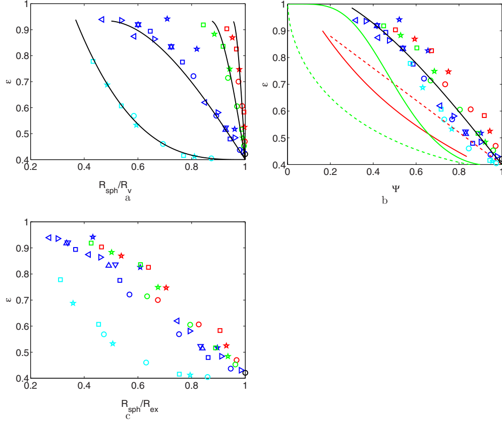
FIG. 6. (Color online) Porosity as a function of R_{sph}/R_v (a), of \Psi (b) and of R_{sph}/R_{ex} (c). Same conventions as in Fig. 5. The black solid lines are model (11) in (a) and Eq. (13) in (b). The solid and broken red lines in (b) are Eqs. (14a) and (14b) with q=2.9 , respectively. The solid and broken green lines in (b) are Eqs. (15a) and (15b), respectively.
