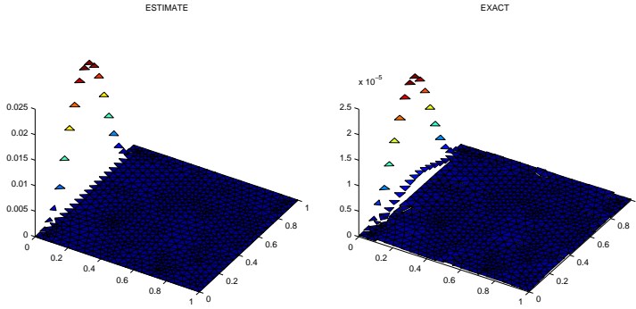
Fig. 8.10 Estimated (left) and exact (right) error distributions for the first-order DG method in the singular test case
