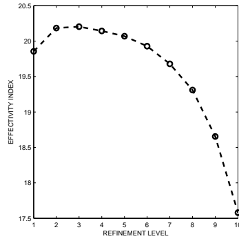
Fig. 8.9 Effectivity indices for the first-order DG method in the singular test case
