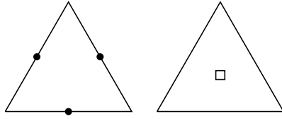
Fig. 7.5 \mathbb{P}_1\text{--}\mathbb{P}_0 nonconforming Crouzeix–Raviart finite elements
