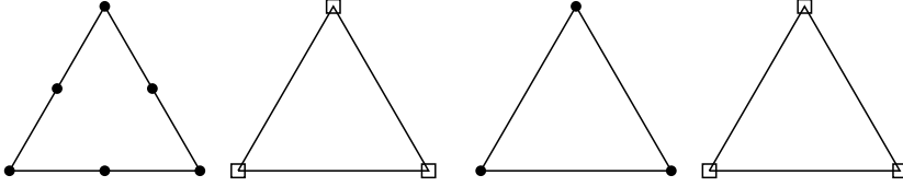
Fig. 7.2 \mathbb{P}_2 - \mathbb{P}_1 Taylor-Hood conforming finite elements (left) and \mathbb{P}_1 - \mathbb{P}_1 stabilized conforming finite elements (right)
