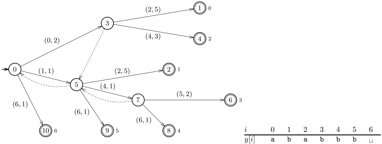
Figure 2: Suffix tree of ababbb . Nodes are numbered in the order of creation. The small numbers closed to each leaf correspond to the position of the suffix associated to the leaf.
