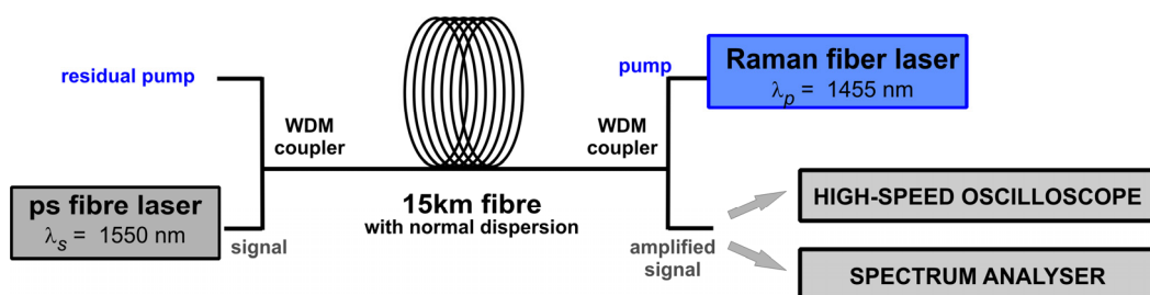
Figure 1 : Experimental set-up
