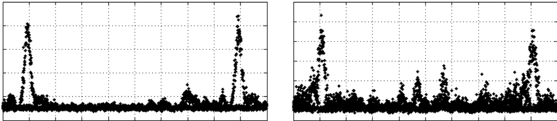
Figure 4. DS-OCDMA signal after decoding (X-axis: 200 ps/div; Y-axis: a.u.). (left): single user; (right): 3 users.
