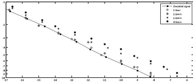
Figure 8. SPE-OCDMA transmission: \log_{10}(BER) vs OSNR (dB).
