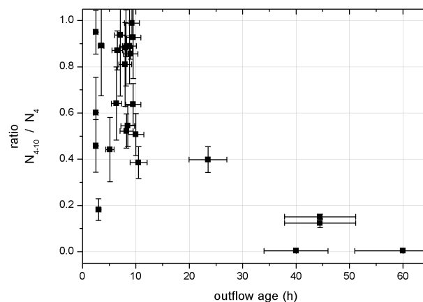
Fig. 17. Mean ratio of the number concentrations of nucleation mode particles (4–10 diameter range; N_{4-10} ) to the total number of particles ( >4 nm; N_4 ) measured in MCS outflow during 26 different cases with varying outflow age between 2.5 and 60 h. Each case represents an average value calculated from typically a few hundred original data points sampled at 1 Hz.
