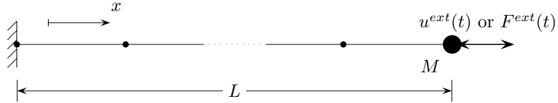
Fig. 3: 1D concrete structure model used for the numerical applications. The cross-section area S = 0.04 \text{ m}^2 , the length L = 1 \text{ m} , the added mass M = 7.0e^5 \text{ kg} , the volumic mass \rho = 2400 \text{ kg.m}^{-3} and the concrete elastic modulus E = 35 \text{ GPa} .
