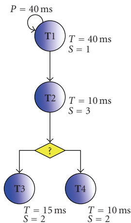
FIGURE 8: Second case: two dynamically chosen tasks.
