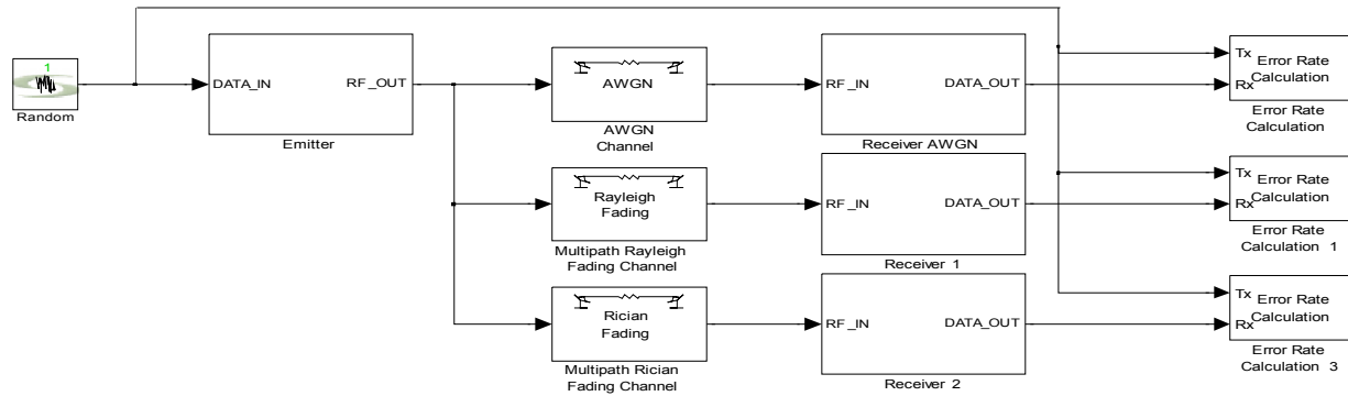
Figure 2. Model for the evaluation of the emitter and the receiver
