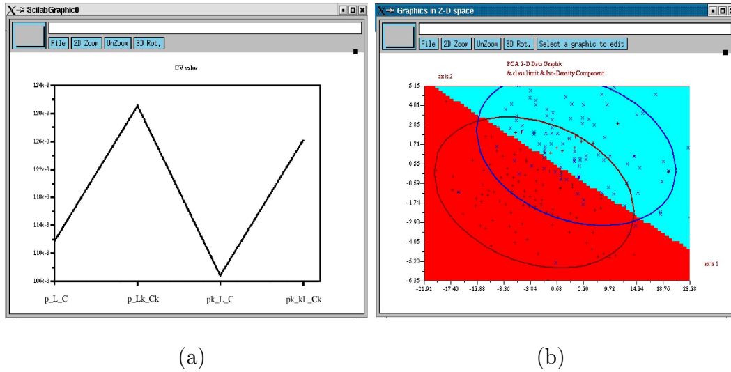
Fig. 5. Selection of a Gaussian mixture model for seabirds: (a) CV values and (b) associated optimal discriminant rule.
