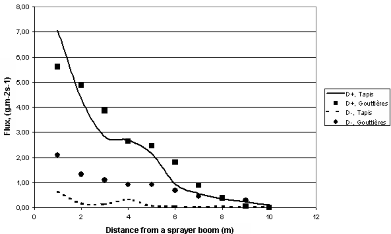
Figure 5. Flow solution trapped on the carpet and in the patternator
