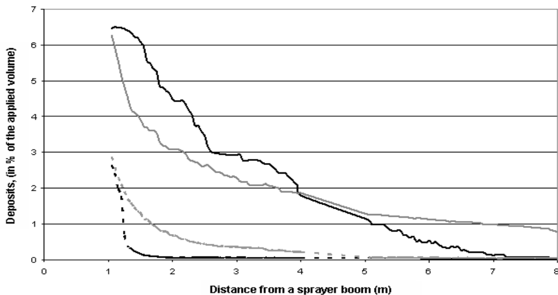
Figure 4. Measuring deposits in wind tunnel for a three nozzles boom XR02; black mark: parallel boom; grey mark: perpendicular boom; continuous mark: drift configuration "D+"; dotted mark: no drift configuration "D-"
