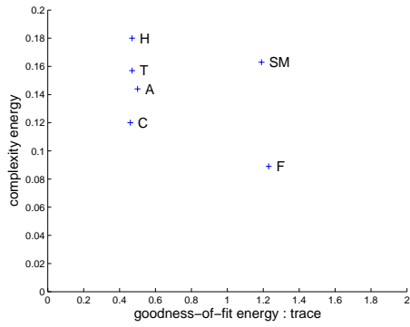
Figure 12. complexity energy versus goodness-of-fit energy : Q for 6 segmentation results of image House.
