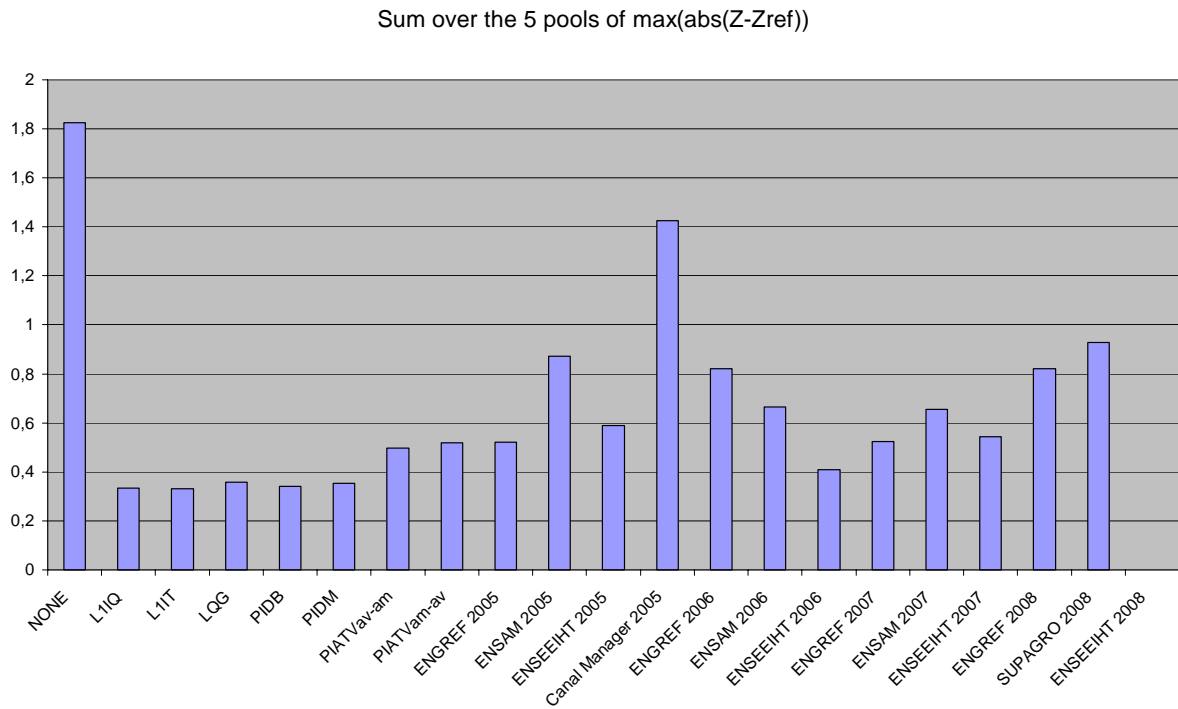
Figure 2. Results of the game for different student groups and automatic controllers (controlled variables)
