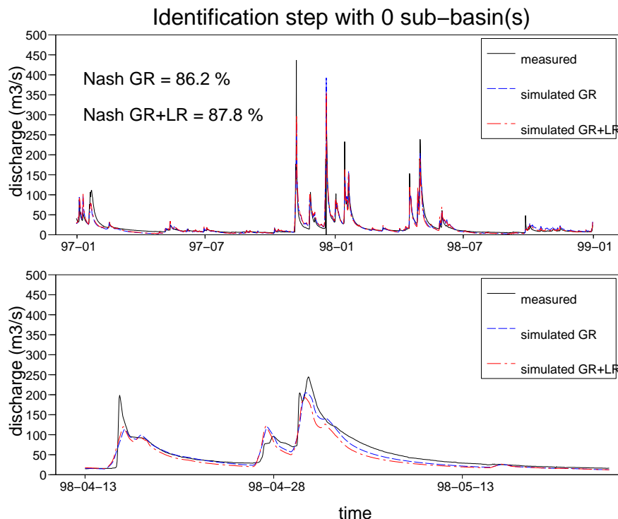
Figure 4: Identification step. Discharge at the downstream end of the channel (on the whole identification period and zoom): (—) measurements, (---) GR simulation, (---) GR+LR simulation without any sub-basin.
