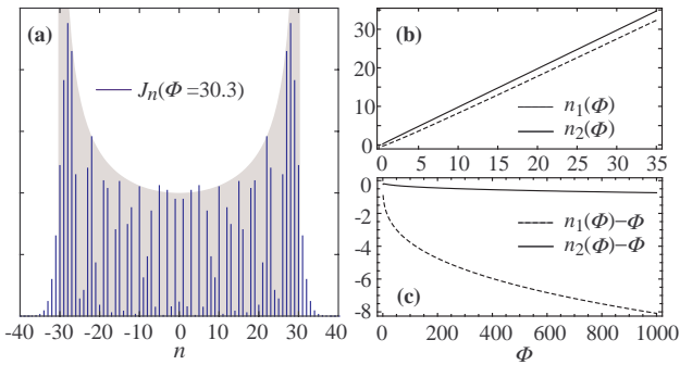
FIG. 1: (a) Relative intensities of the sidebands as a function of n for fixed \Phi = 30.3 rad. The vertical lines show the intensities of the discrete n components of the real spectrum. The light grey shade shows the Doppler spectrum obtained from the vibration velocity distribution, with a continuous variable on the horizontal axis n = (\nu - \nu_0)/\nu_A . Both spectra fall abruptly beyond n = \pm 30.3 , which corresponds to the Doppler shift associated with the maximum velocity. (b) The broken line shows the values n_1 as a function of \Phi , where n_1 is the value of n giving the maximum intensity in the discrete spectrum; the full line shows n_2 , where n_2 is the value of n for which the intensity is half the maximum, which gives a very good approximation of \Phi . (c) The broken and full lines respectively show n_1 - \Phi and n_2 - \Phi as a function of \Phi .
