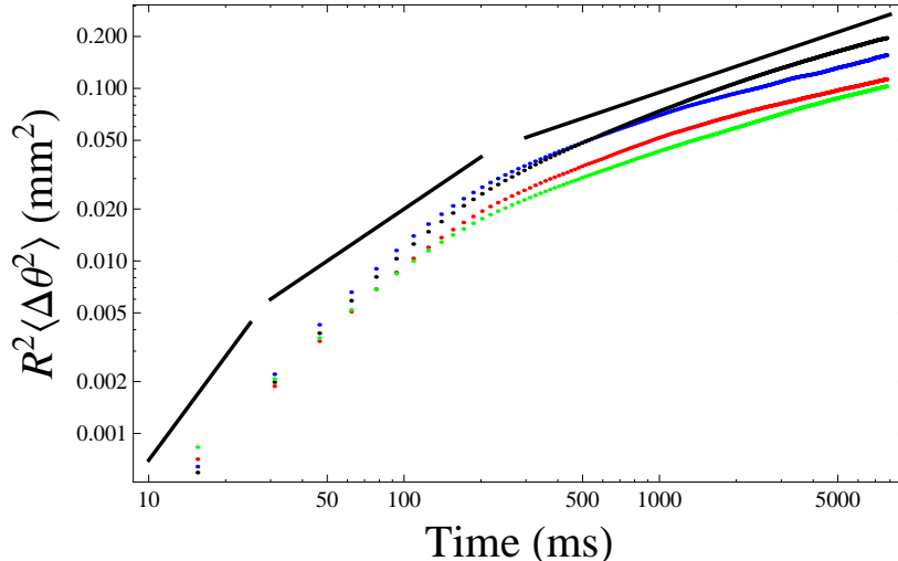
FIG. 8: (Color online) Plot of the orthoradial m.s.d. R^2\langle\Delta\theta^2\rangle (in \text{mm}^2 ) as a function of time t (in ms), in a log-log scale, for densities 477 \text{ m}^{-1} (blue dots, small annulus, N = 12 ; black dots, large annulus, N = 27 ) and 637 \text{ m}^{-1} (red dots, small annulus, N = 16 ; green dots, large annulus, N = 37 ). The solid black lines are of slopes 2, 1 and 1/2 . The temperature is the same in all experiments ( T = 11.2 \cdot 10^{11} \text{ K} ) and the applied voltage is 1000 V. The crossover time decreases when the density increases.
