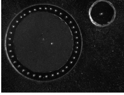
FIG. 3: Picture of the circular channel with N = 37 beads inside, recorded during an experimental run ( T = 10.2 \cdot 10^{11} K, V_0 = 1000 V). Inner radius 8 mm, outer radius 10 mm, beads diameter 0.8 mm. In the right-up corner, an identical bead confined in a disk of radius 5 mm is the embedded thermometer.
