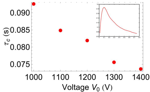
FIG. 9: (Color online) Crossover time \tau_C (in s.) as a function of the applied voltage (in V.) In the inset we plot the m.s.d. divided by the time as a function of the time. The crossover time is estimated as the position of the maximum of this curve.
