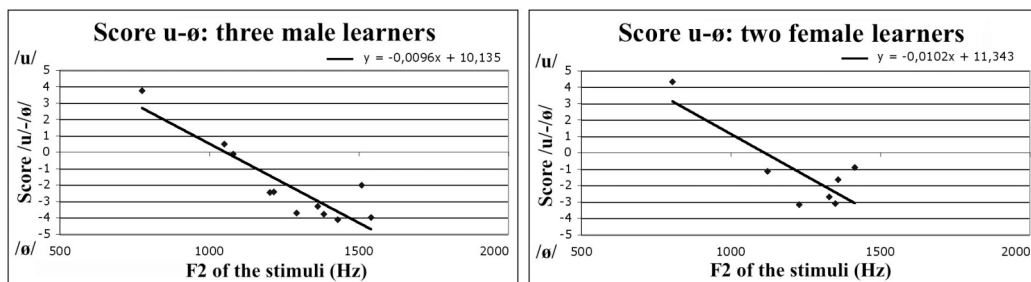
Figure 16 F2 of the stimuli (x-axis) and the index “u-ø” score (y-axis) for stimuli pronounced by 3 male learners (left) and 2 female learners (right). 64 responses (4 repetitions x 16 NF listeners) for each stimulus.
