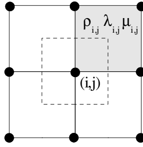
Figure 1. Illustration of grid structure and material properties distribution. Dashed line indicates the control element used in calculations.
