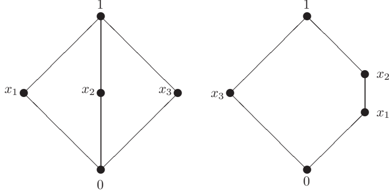
FIGURE 1. The lattices M_3 and N_5 .
