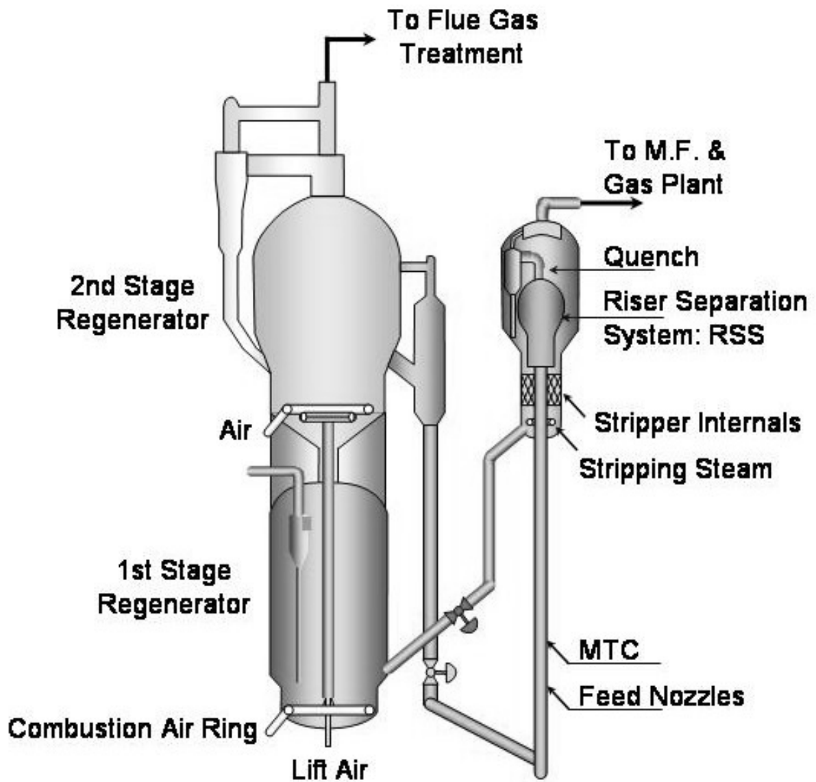
Figure 1 : The R2R resid Fluid Catalytic Cracking process (Axens-IFP-Stone & Webster Inc.-
