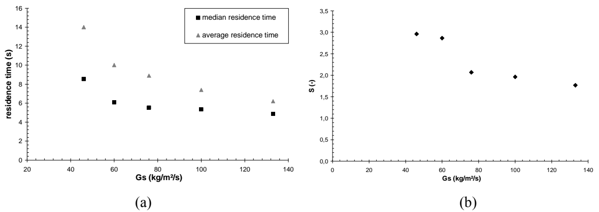
Figure 12. Residence time (a) and spread coefficient (b) evolutions with the solid flux
