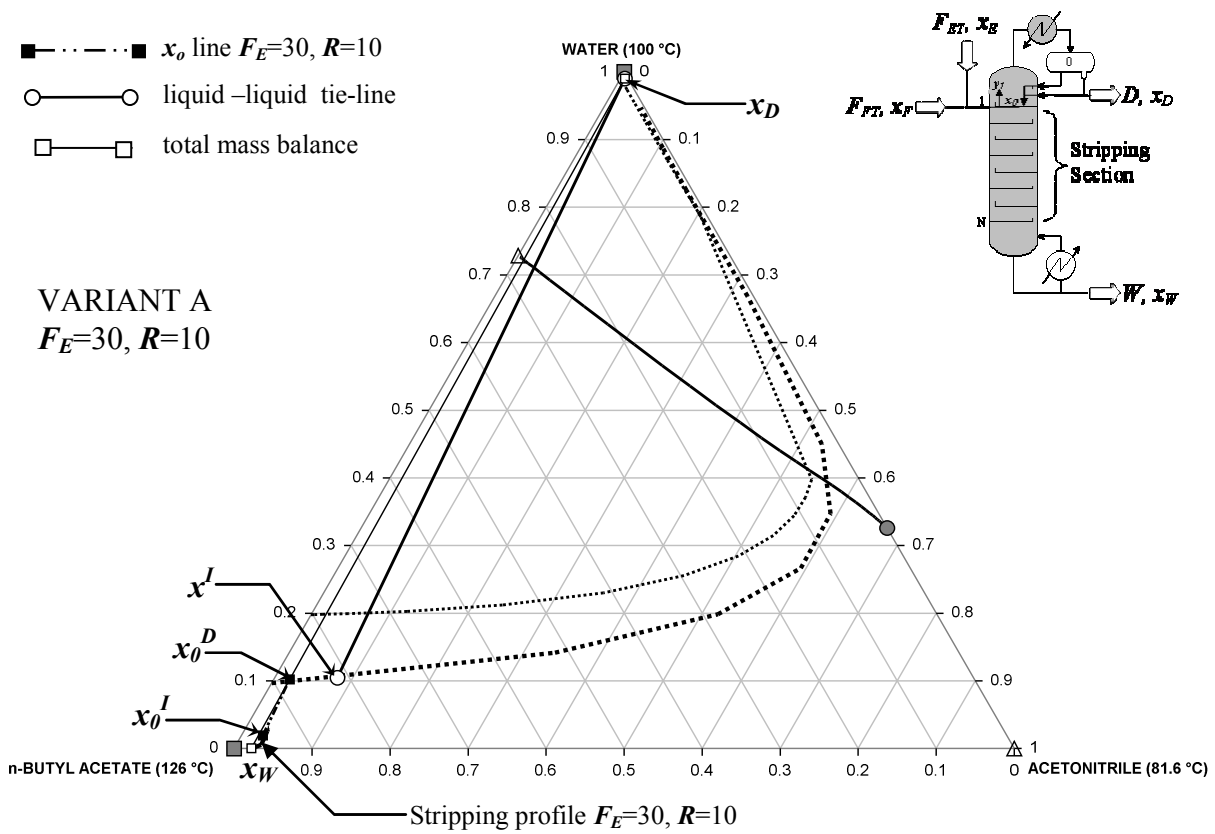
Figure 9. Stripping composition profile and line of valid value of x_0 for variants A, B and C for column configuration 4.
