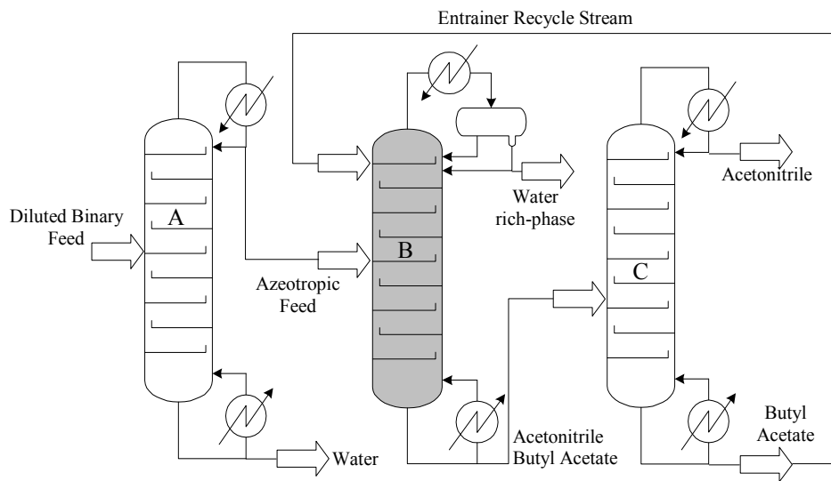
Figure 2. Typical column sequence for the heterogeneous continuous distillation process. (A) Pre-concentrator, (B) Heterogeneous Distillation Column, (C) Entrainer Recovery Column.
