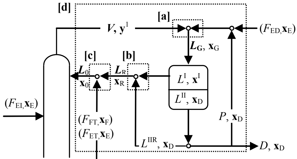
Figure 4. Combined options for entrainer recycle stream and the main azeotropic feed stream in the top part of the heterogeneous column considering that they can be supplied to the decanter or mixed with the reflux.
