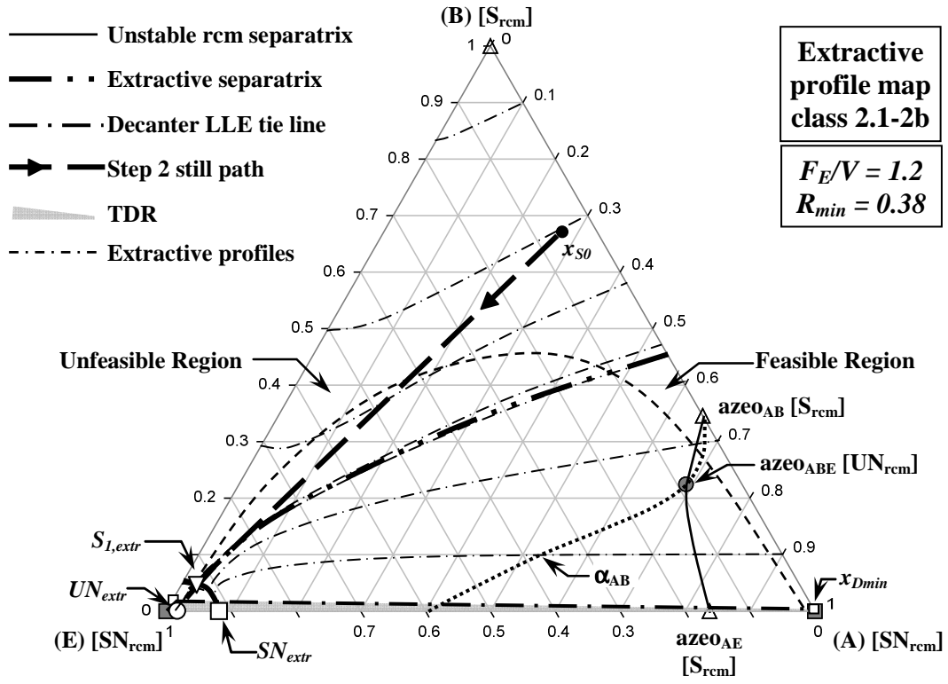
Fig. 6. Extractive liquid profiles map ( (F_E/V)=1.2 ; R_{min}=0.38 ).
