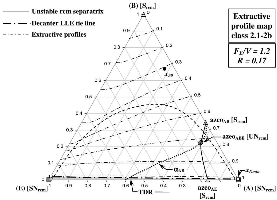
Fig. 7. Extractive liquid profiles map ( (F_E/V)=1.2 ; R=0.17 ). Unfeasible region matches the whole triangle.
