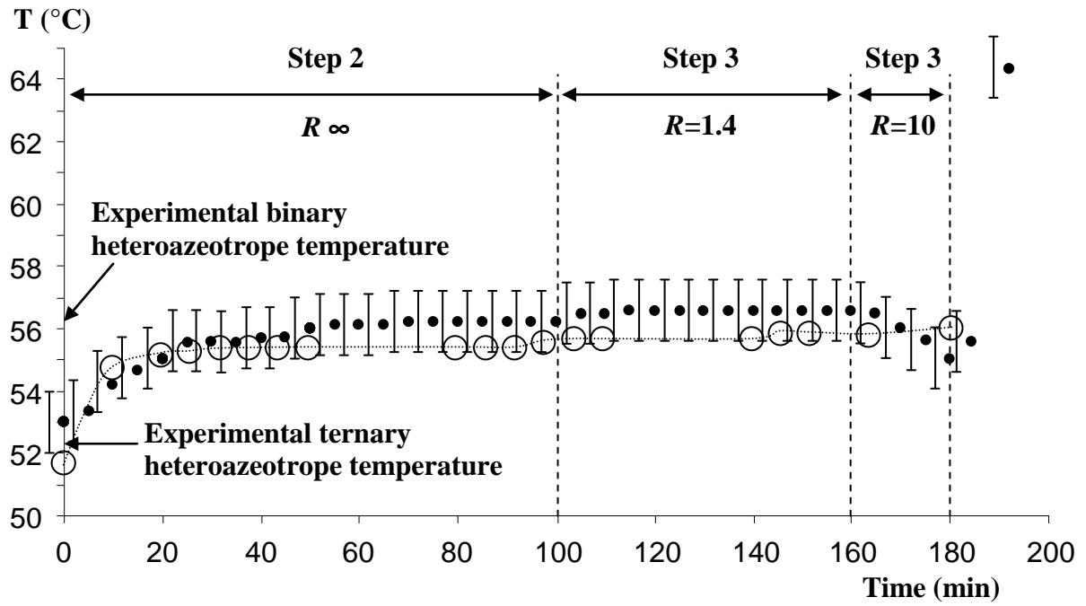
Fig. 10. Top temperature evolution for the six experimental replicates and simulation results of the heterogeneous extractive distillation process in a batch rectifying column. Experimental results ( ● ). Simulation results ( ○ )
