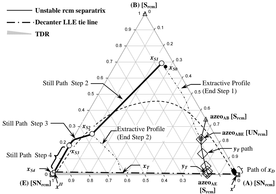
Fig. 8. Simulation results of the separation of chloroform – methanol with water by heterogeneous extractive batch distillation process.
