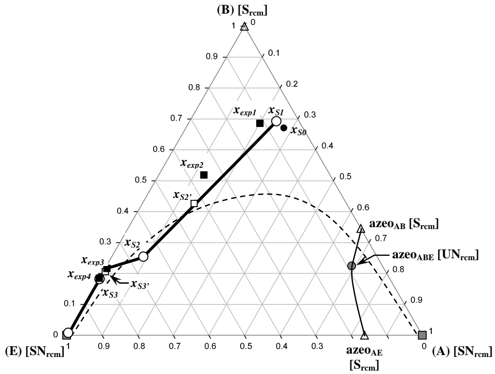
Fig. 9. Simulation and experimental results of the separation of chloroform – methanol with water by heterogeneous extractive distillation process in a batch rectifying column.
