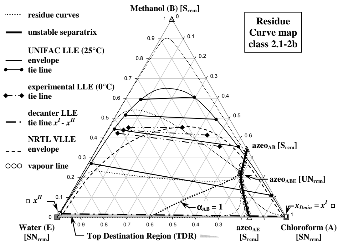
Fig. 1. Chloroform (A) – Methanol (B) – Water (E) residue curve map (class 2.1-2b)
