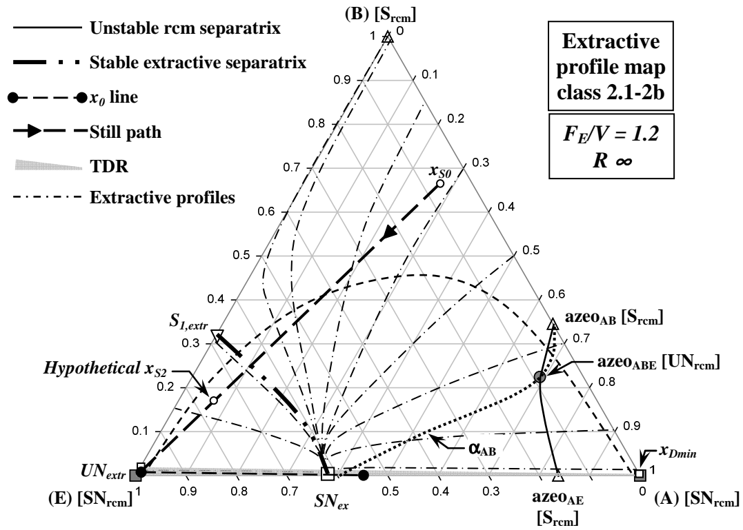
Fig. 4. Extractive liquid profiles map ( (F_E/V)=1.2 ; infinite reflux) (step 2).
