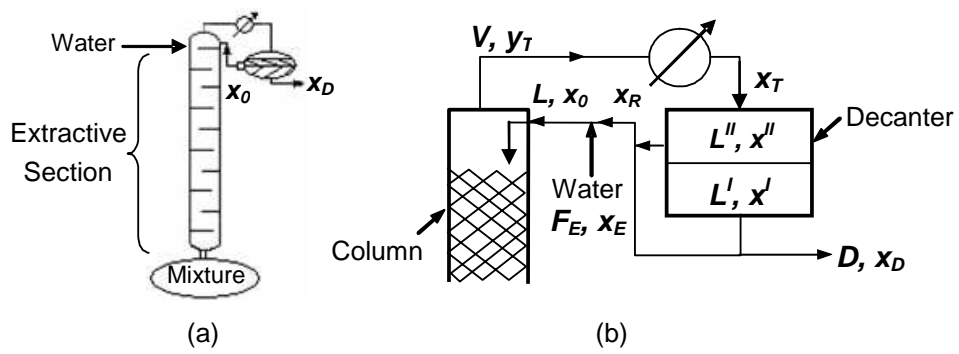
Fig. 2. Batch rectifying column configuration for heterogeneous extractive distillation (a) column. (b) column top and decanter details.
