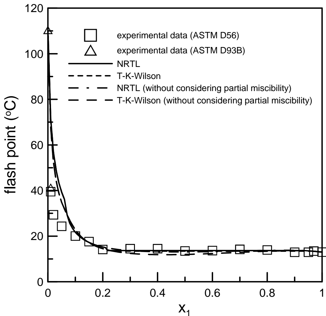
Fig. 6. Comparison of predicted flash point and experimental data for ethanol (1) + tetradecane (2).
