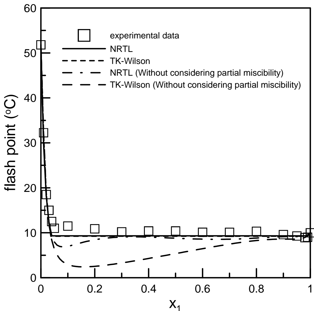
Fig. 3. Comparison of predicted flash point and experiment data for methanol (1) + decane (2).
