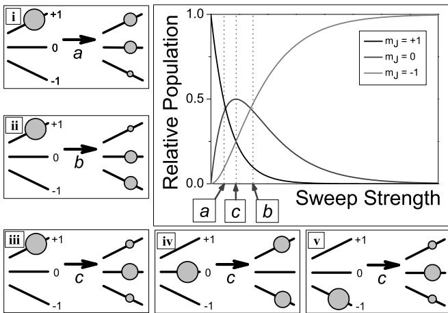
FIG. 3: RF sweep schemes. The large panel shows the solution to the three level L-Z system for input state m_J = 1 , plotted vs. “Sweep Strength” which is proportional to the RF power for a sufficiently broad sweep of fixed duration. Panels [i-v] show the effects of ramps of various strengths (labeled “a”, “b”, and “c”) on different input states. Note that the total population is an incoherent mixture of spin states, so only single state inputs are considered. Panels [i-iii] correspond directly to the main panel, and [v] is equivalent to [iii] with the m_J = \pm 1 states reversed. The behavior of panel [iv] can not be inferred from the main panel, since the input state in this case is m_J = 0 , though we have confirmed the result both experimentally and numerically, as described in the text.
