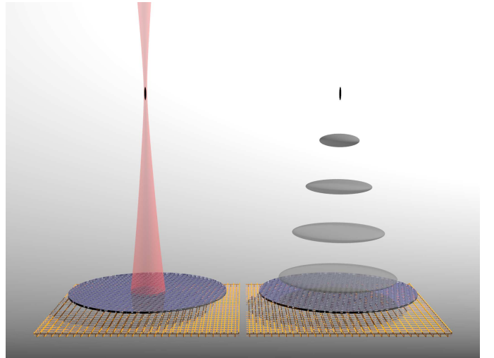
FIG. 1: Trap and detector layout. The optical trap is formed from a vertically propagating red-detuned beam. The anisotropy of the potential results in a vertically elongated condensate with typical radial and axial (vertical) Thomas-Fermi radii of R_r \sim 2.5 \mu\text{m} , and R_z \sim 600 \mu\text{m} , where R_i^2 = 2\mu_{3D}/m\omega_i^2 (the 3D chemical potential \mu_{3D} is defined in the text, and trap frequencies \omega_i corresponding to a BEC are given in the following figure caption). After release from the trap, during the 300 ms TOF, the condensate expands into a horizontally oriented “pancake” distribution since the radial size increases by a factor of \sim 3000 , while the axial size increases by only a few percent. After their TOF, individual atoms are detected in the horizontal plane with a crossed delay line anode positioned beneath an MCP. Combined with the time of arrival, this allows a 3D reconstruction of the TOF atomic distribution.
