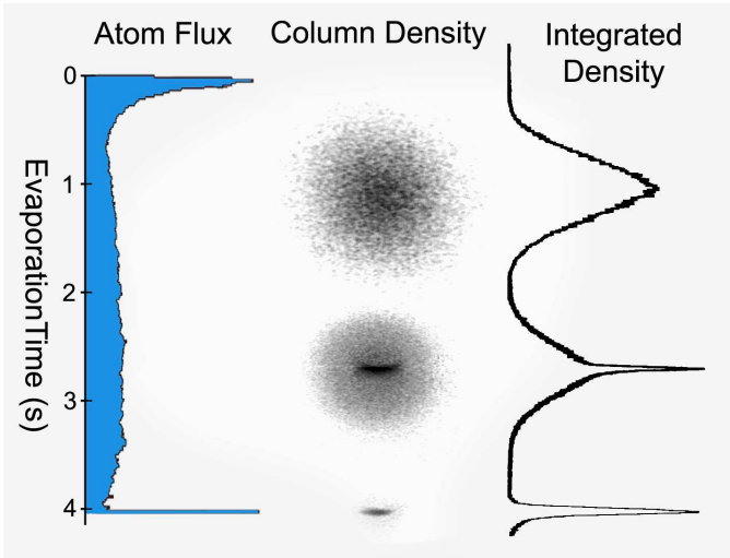
FIG. 2: Evaporation to BEC. On the left is the flux of atoms exiting the trap over the vertical potential lip during evaporation. These atoms remain confined by the trapping beam in the horizontal plane, and so are guided onto the MCP. The peak near time = 0 s is associated with atoms lost during transfer from the magnetic trap and the subsequent rapid thermalization of the remaining atoms. The peak near 4 s is the TOF density distribution of the cold atoms released at the end of evaporation. In the center are 2D column densities obtained by integration along one horizontal axis of the 3D TOF density distributions of released clouds of various temperatures. On the right are the corresponding axial profiles made by integration along the remaining horizontal axis. At full trap depth, the temperature T = 3 \mu\text{K} > T_c , where the critical temperature for condensation T_c \approx 2 \mu\text{K} , and so the momentum distribution is thermal (top). As the temperature is lowered below T_c , the distribution becomes a bimodal superposition of thermal and condensed atoms, marked by the high visibility of the pancake shaped condensed fraction contrasted with the uniformly distributed thermal component (middle). When the trap intensity is lowered until I \approx 0.5 I_o , the temperature T \ll T_c , and the thermal component is removed, leaving a quasi-pure condensate of up to N = 10^5 atoms with condensed atom fraction N_c/N \geq 0.9 (bottom). At this trap depth ( U_{eff}/k_B \sim 0.25 \mu\text{K} ), the trap frequencies are \omega_r/2\pi = 1.5 \text{ kHz} and \omega_z/2\pi = 6.5 \text{ Hz} .
