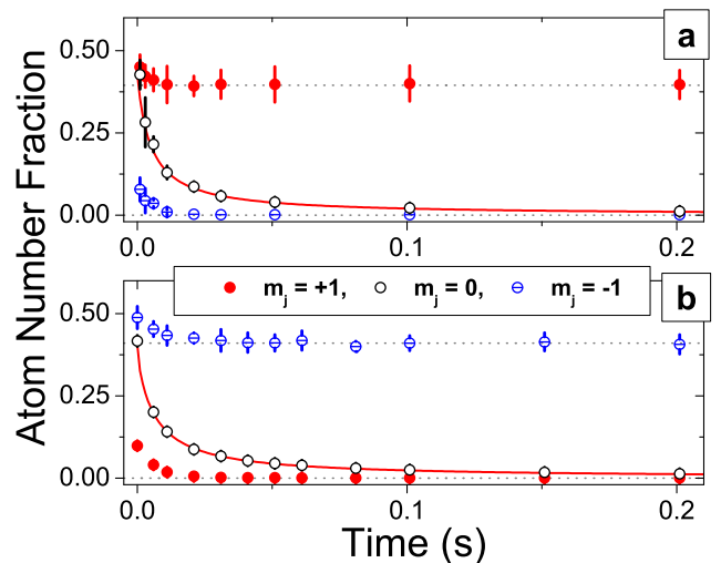
FIG. 4: Loss processes in imbalanced mixtures. Two initial spin state populations prepared using “a” and “b” of fig. 3 are plotted vs. time to determine the stable and unstable spin combinations. The error bars correspond to the standard deviation of the mean derived from repeated measurements. The solid curve through the m_J = 0 points is a fit to a two-body loss process corresponding to a preliminary value \beta_{00}^{prelim} \approx 7 \times 10^{-10} \text{ cm}^3/\text{s} , and is shown for reference, since in this case, systematic uncertainties in atom number and temperature that result from residual distortions associated with the Stern-Gerlach field limit the precision of the measurement. The dotted horizontal lines are shown for reference.
