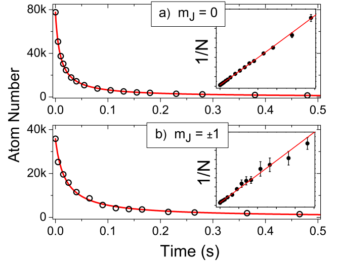
FIG. 5: Loss of m_J = 0 and m_J = \pm 1 atoms. The population of m_J = 0 or the m_J = \pm 1 atoms are separately measured to refine measurements of the respective loss rate constants \beta_{00} and \beta_{\pm 1} . Error bars, corresponding to the standard deviation of the mean, are equivalent to or smaller than the data point symbols (on the linear scale). The curves show the best fit to a two-body decay process for a thermal bose gas in the true optical plus gravitational potential, including the measured one-body loss rate, as described in the text. The insets show the same data and fits plotted as 1/N vs. time. When plotted in this way, the decay resulting from purely two-body processes appears linear with time, and so the linearity of the data exemplifies the limited contribution of one and three-body loss processes.
