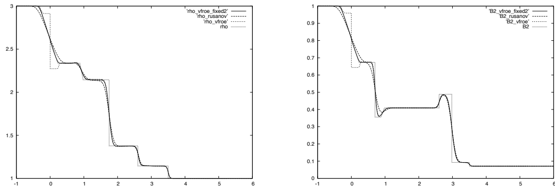
Figure 2. Test case 2: density and second component of the magnetic field. Comparison between the VFRoe-ncv scheme, the VFRoe-ncv scheme with the parameter-free entropy fix and the Rusanov scheme.
