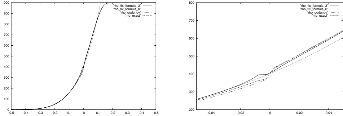
Figure 1. Test case 1: density profiles obtained by using 200 cells. Comparison between Godunov, VFRoe with two fixes and the exact solution. A zoom on the density profiles around the sonic point is displayed on the right.
