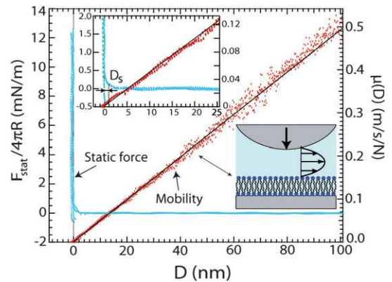
Fig. 3 Static force F_{stat} and sphere mobility as a function of the sphere-plane distance, obtained on a DPPC bilayer. The sphere radius is R = 2.9 \pm 0.3 μm and the frequency 19 Hz. The straight line is the best fit of the damping.
