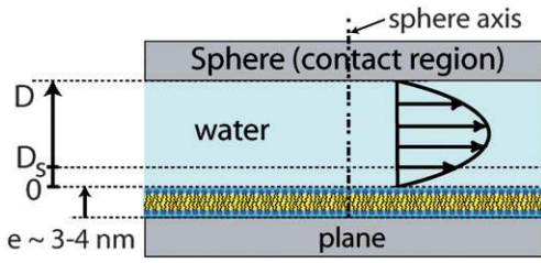
Fig. 4 Schematic representation of the flow of water on a DPPC bilayer and the associated distances. The origin of distances corresponds to the hydrodynamic contact between the sphere and the bilayer. The onset of the steric repulsion occurs at the distance D_s = 1 \pm 0.5 nm from hydrodynamic contact, through a fluid water film of similar viscosity as bulk water.
