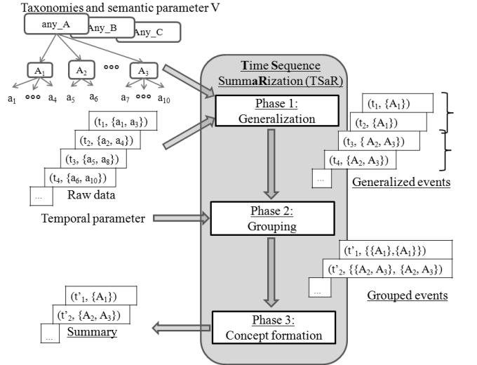
Figure 1: TSaR summarization process
