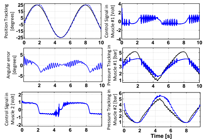
Fig. 10. Dynamic tracking test for the muscles with the attached arm and for high angle ranges ( +/-25^\circ )
