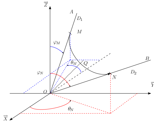
Figure 5: Parametrization of passage of discontinuity
