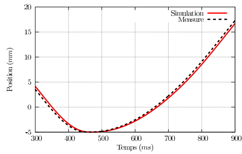
Figure 11: Passage of a discontinuity in a curvature
