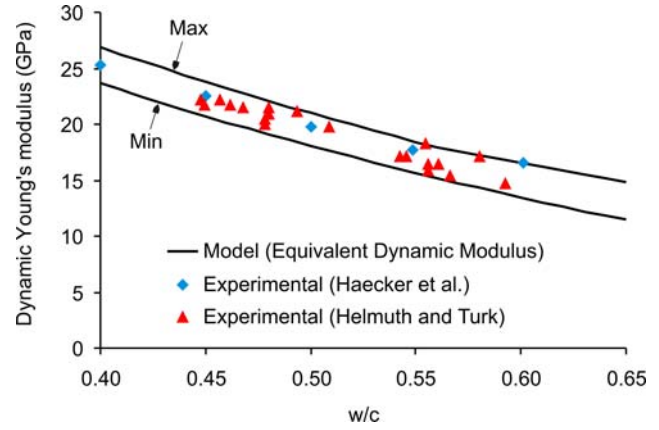
Figure (4): Comparison of the predicted drained Young's modulus and the experimental results of Helmuth and Turk [62] and Haecker et al. [61]. The static elastic modulus predicted by the model is converted into a range of equivalent dynamic modulus using the empirical relation (61) and the calibration parameters from Hana and Kim [68].
