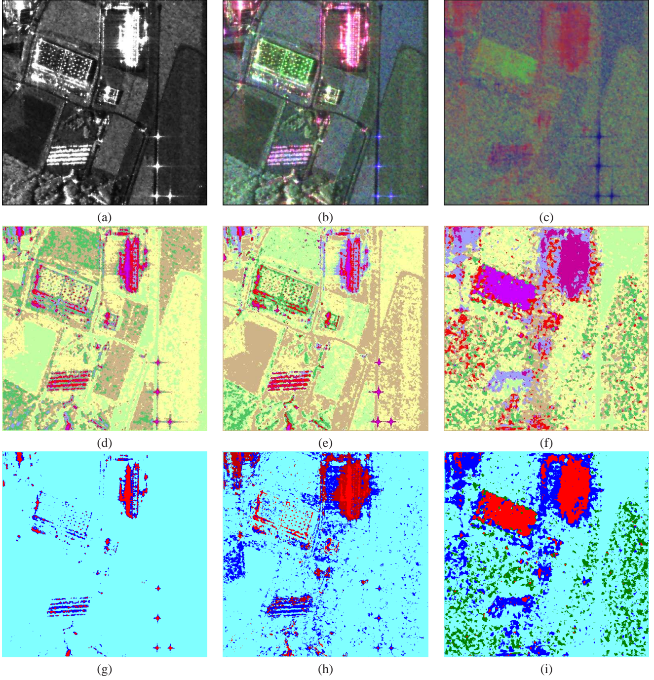
Fig. 9. Brétigny, RAMSES POLSAR data, X-band (501 × 501 pixels). LLMMSE span using the normalized coherency estimated by SDAN-FP: (a) span image, (d) Gamma unsupervised classification and (g) physical mechanism identification (odd bounce classes, even bounce classes, volume class) using the SDAN-FP normalized coherency. SDAN-FP coherency matrix after span multiplication: (b) color composition of the diagonal elements [T]_{11} - [T]_{33} - [T]_{22} , (e) Wishart unsupervised classification and (h) physical mechanism identification. SDAN-FP normalized coherency matrix: (c) color composition of the diagonal elements [M]_{11} - [M]_{33} - [M]_{22} , (f) SIRV unsupervised classification and (i) physical mechanism identification.
