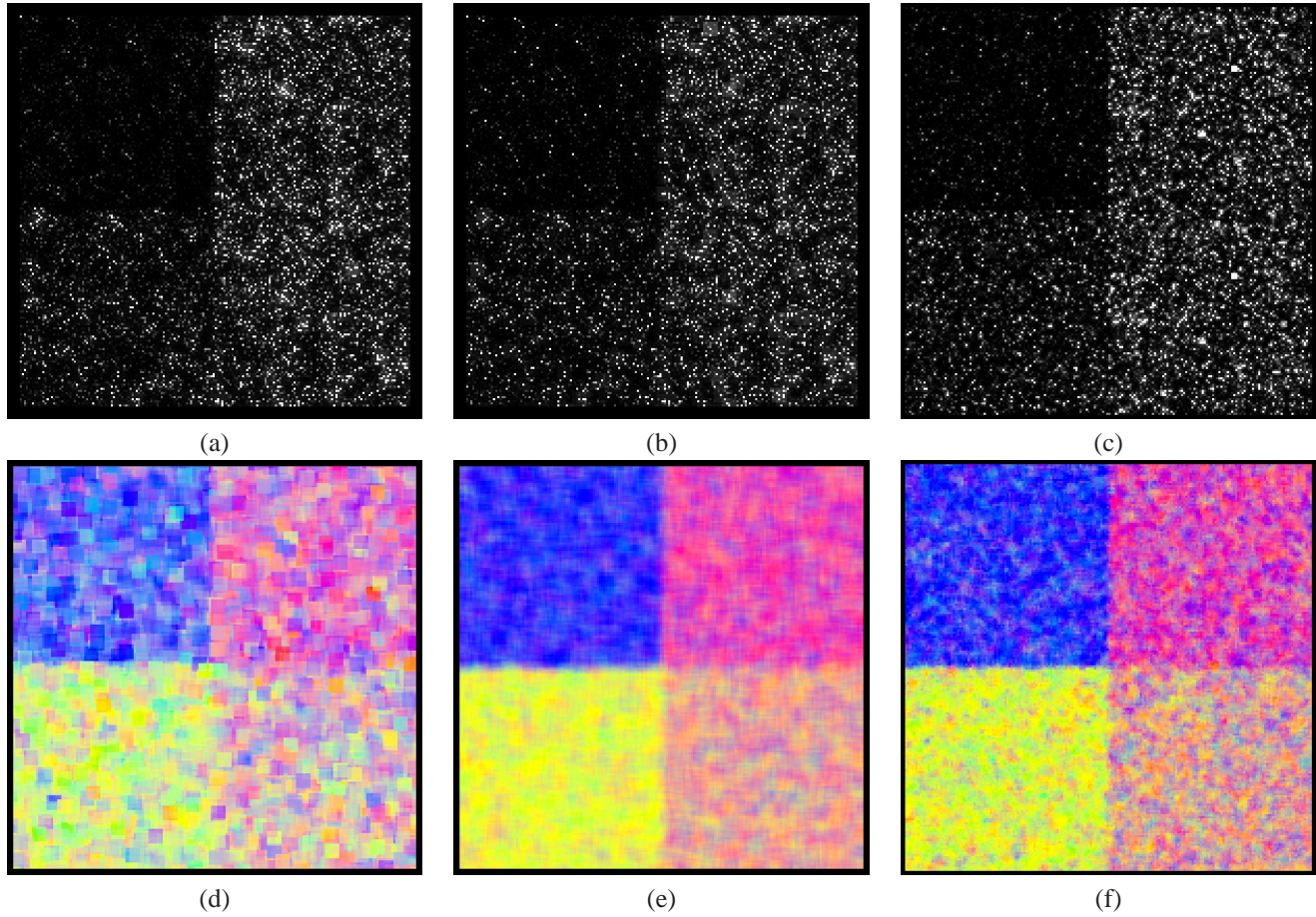
Fig. 5. Simulated POLSAR data, SIRV case ( 200 \times 200 pixels). Square root of LLMMSE span image using the normalized coherency estimated by: (a) BN-SCM, (b) BN-FP and (c) SDAN-FP. Color composition of the normalized coherency diagonal elements [M]_{11} - [M]_{33} - [M]_{22} estimated by: (d) BN-SCM, (e) BN-FP and (f) SDAN-FP.
