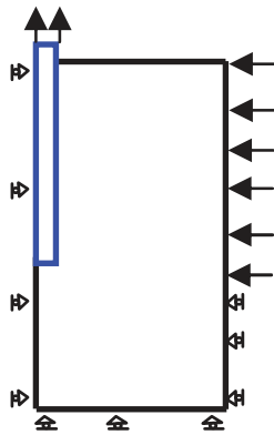
Figure 1: Pull-out of a pile
