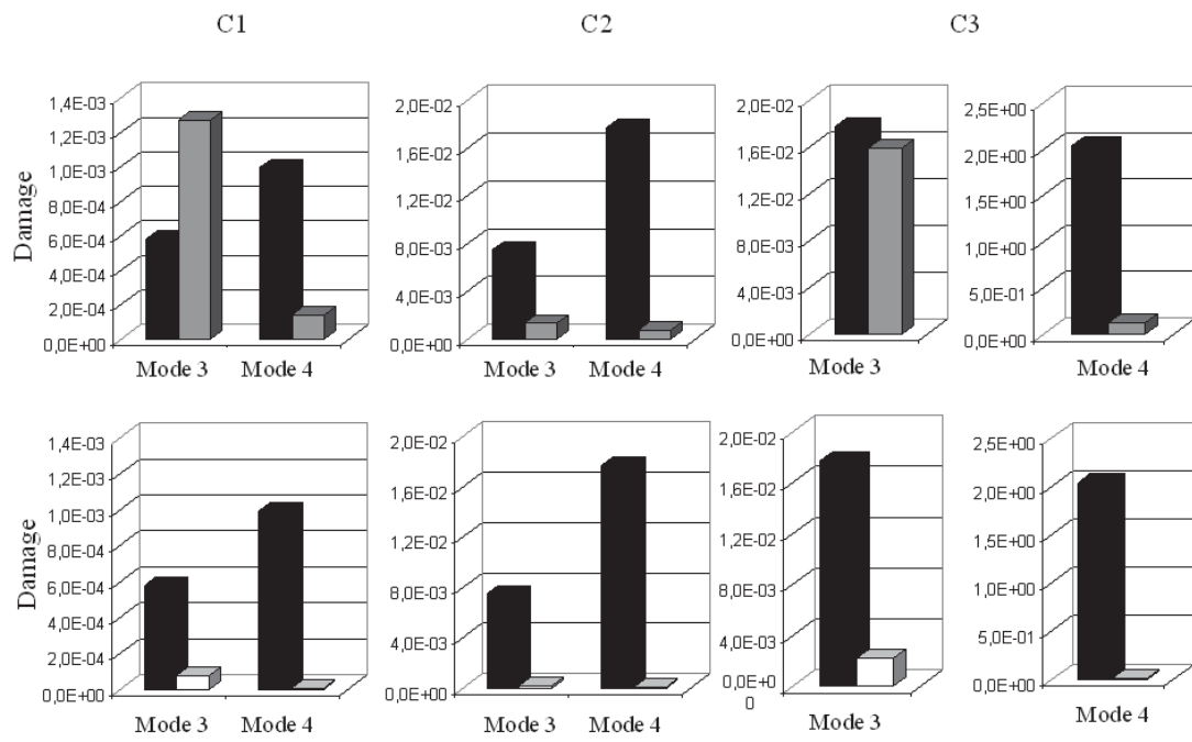
Fig. 16. Damage reduction with LQG control calculated with CirVibe® (■ uncontrolled PCB without piezoelectric components, ■ controlled PCB with activated piezoelectric components).
