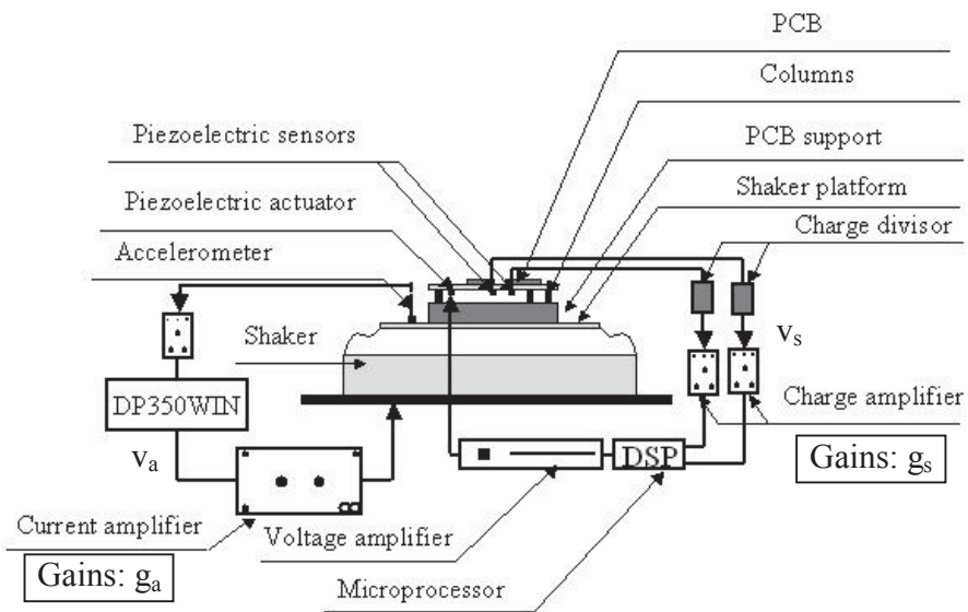
Fig. 9. Experimental set-up.
