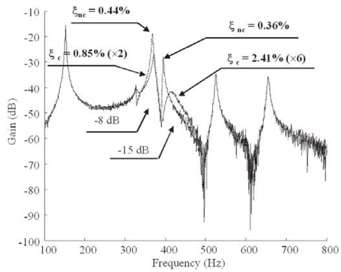
Fig. 10. Experimental uncontrolled (···) and controlled (—) FRF between the accelerometer and the first piezoelectric sensor for a 1\text{ g}_{\text{rms}} disturbance.
