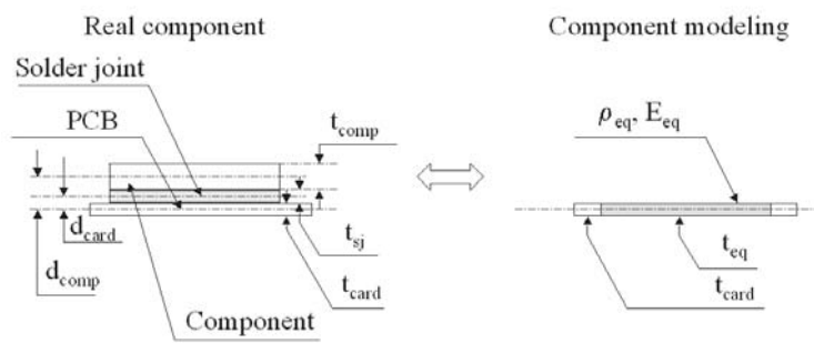
Fig. 4. Component modelling.
